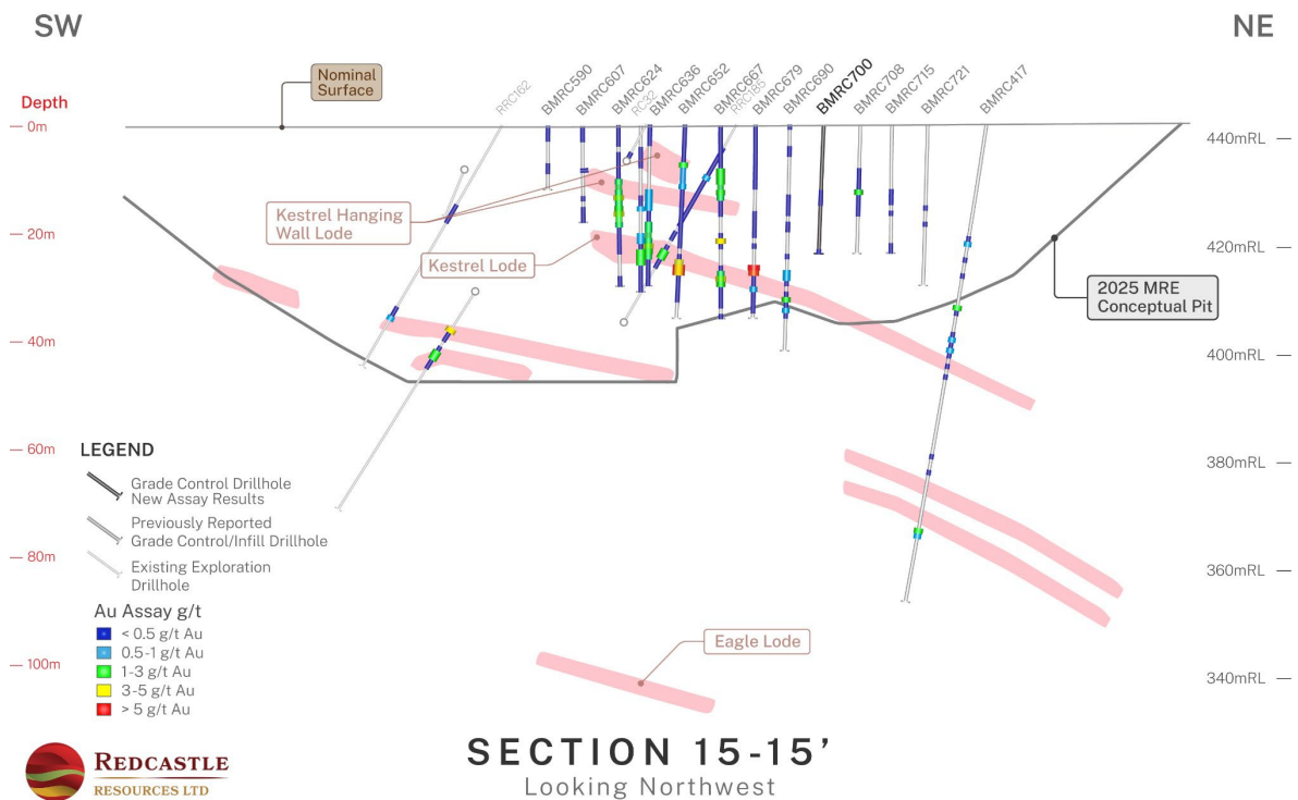
Figure 16. Queen Alexandra Section 15-15'
