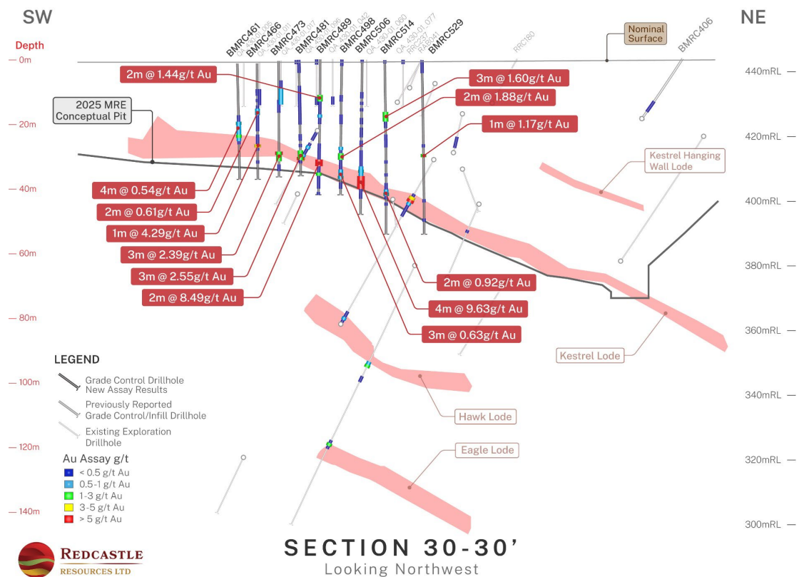
Figure 29. Queen Alexandra Section 30-30'
