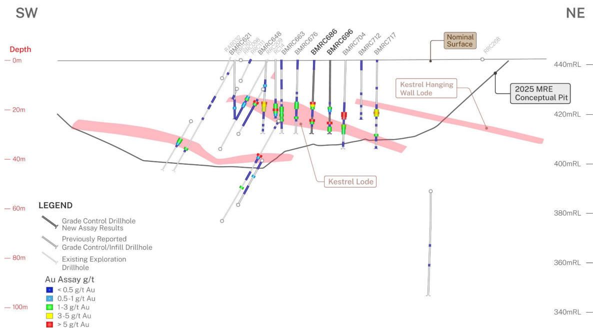
Figure 12. Queen Alexandra Section 11-11'
