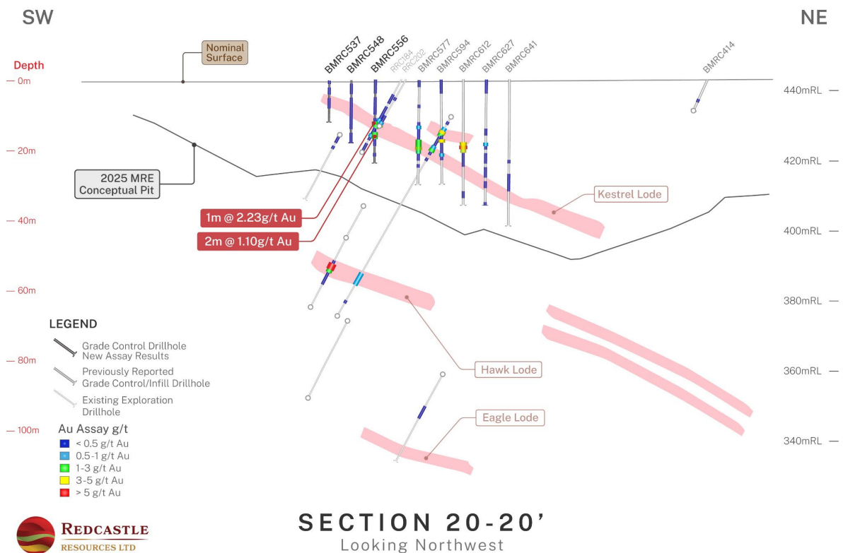
Figure 21. Queen Alexandra Section 20-20'
