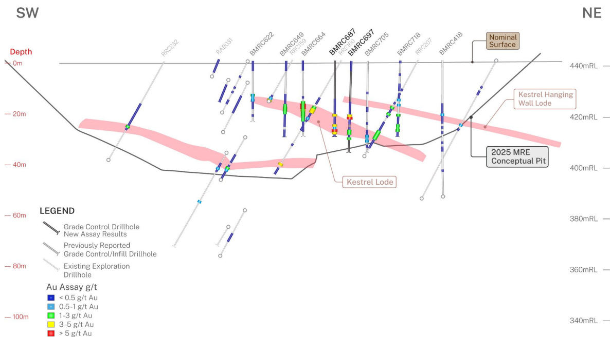
Figure 13. Queen Alexandra Section 12-12'
