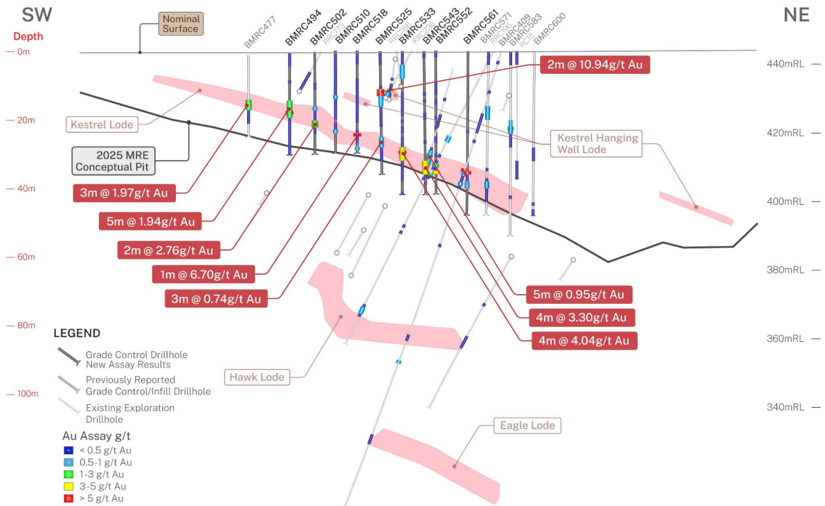
Figure 26. Queen Alexandra Section 26-26'
