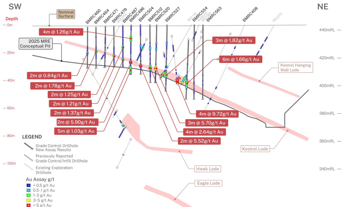
Figure 26. Queen Alexandra Section 26-26'
