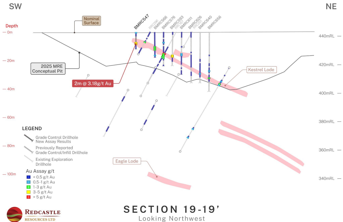
Figure 20. Queen Alexandra Section 19-19'
