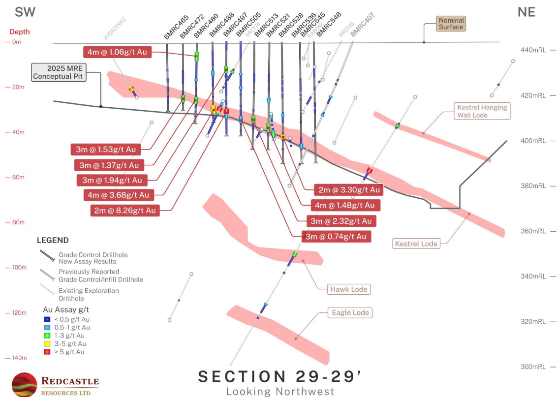
Figure 28. Queen Alexandra Section 29-29'
