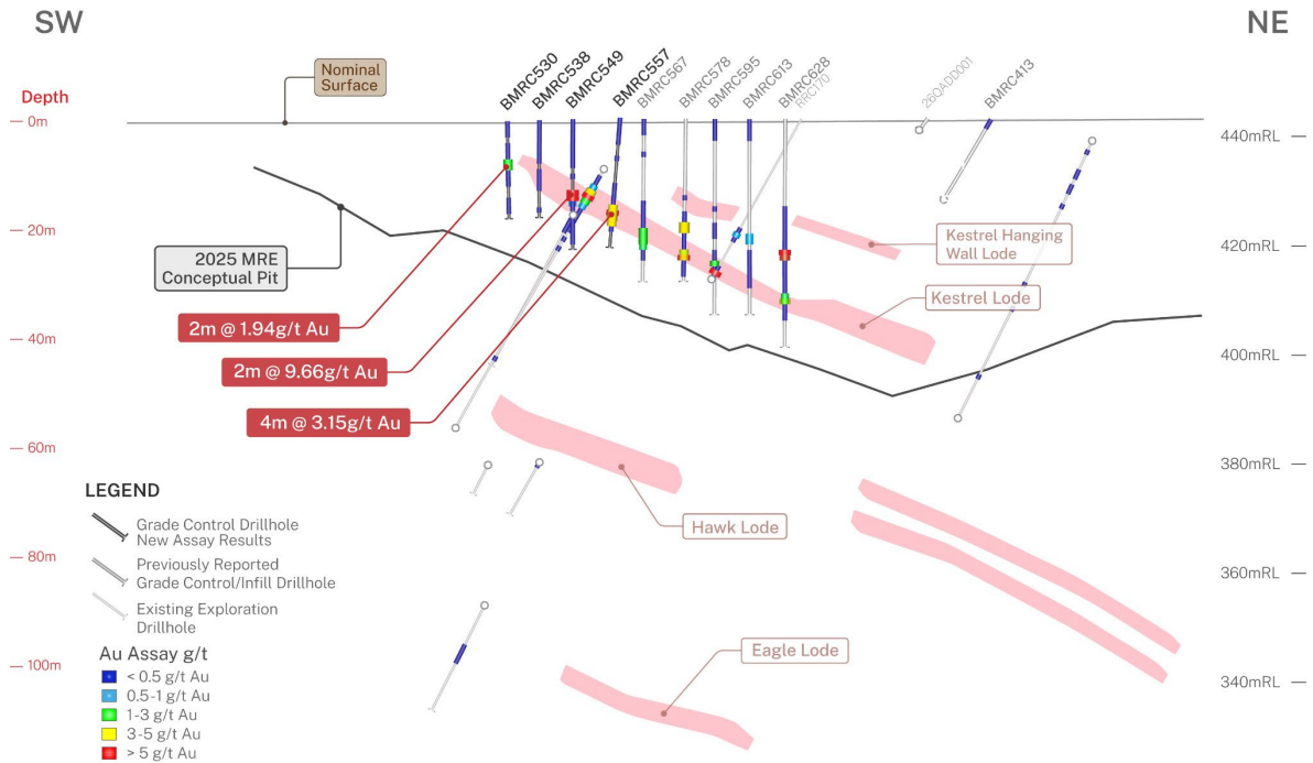
Figure 22. Queen Alexandra Section 21-21'
