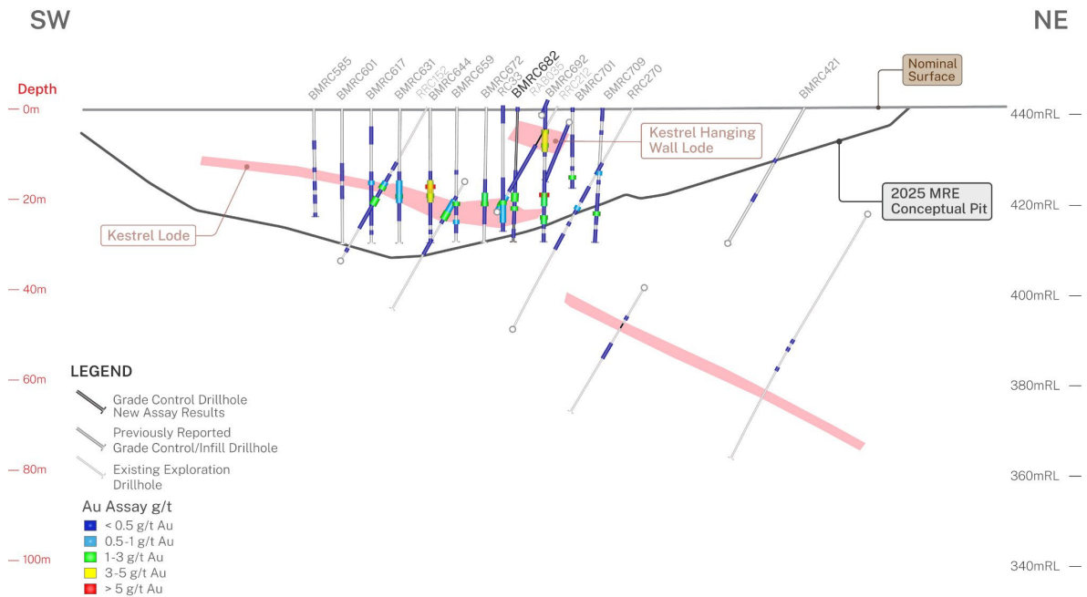
Figure 8. Queen Alexandra Section 7-7'
