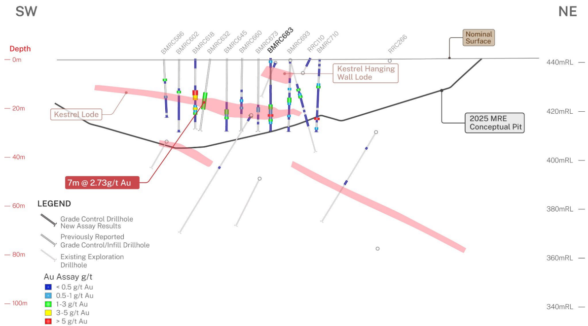
Figure 9. Queen Alexandra Section 8-8'
