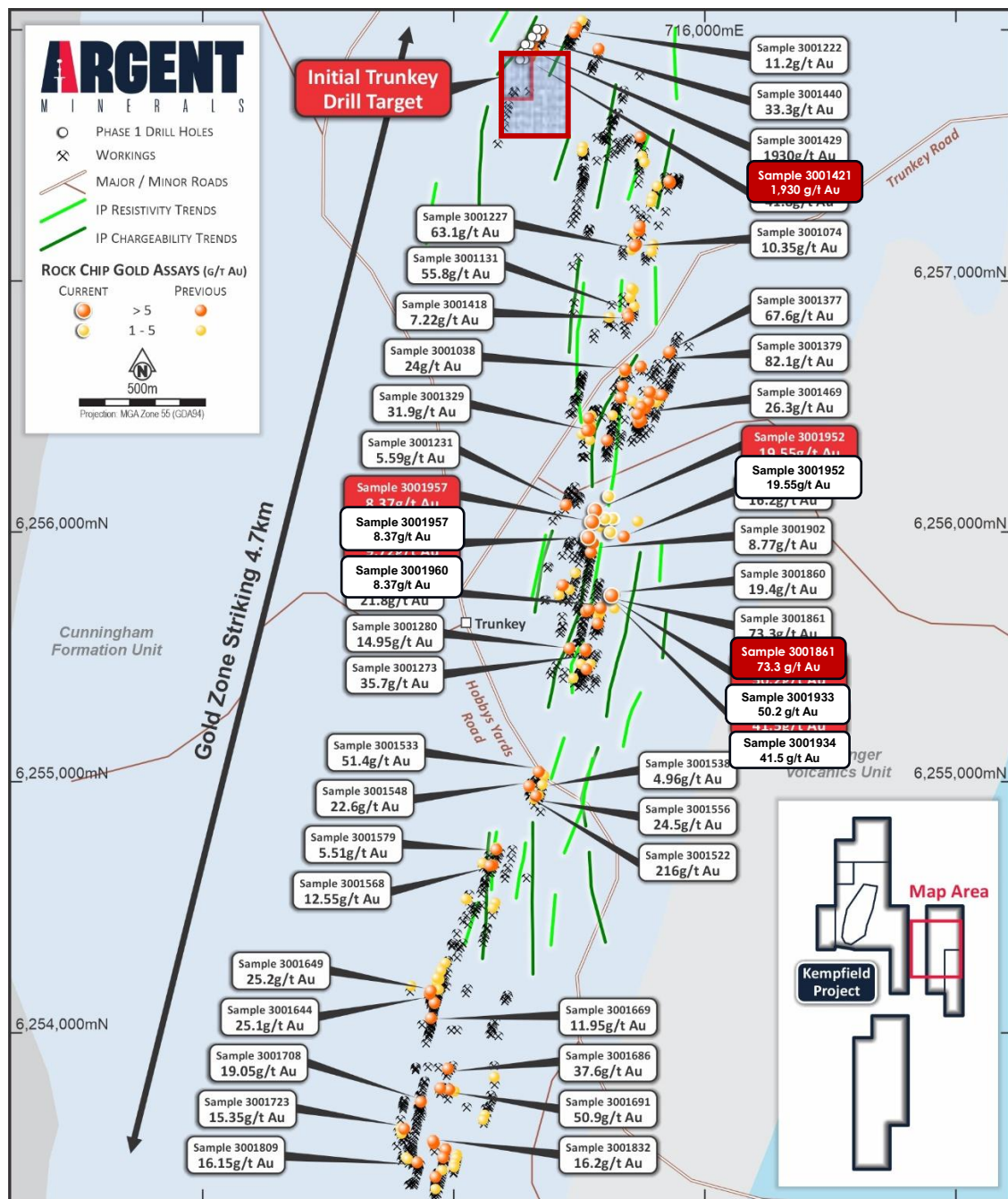
Figure 5. Rock chip sample results from earlier program in relation to Phase 1 drilling.
