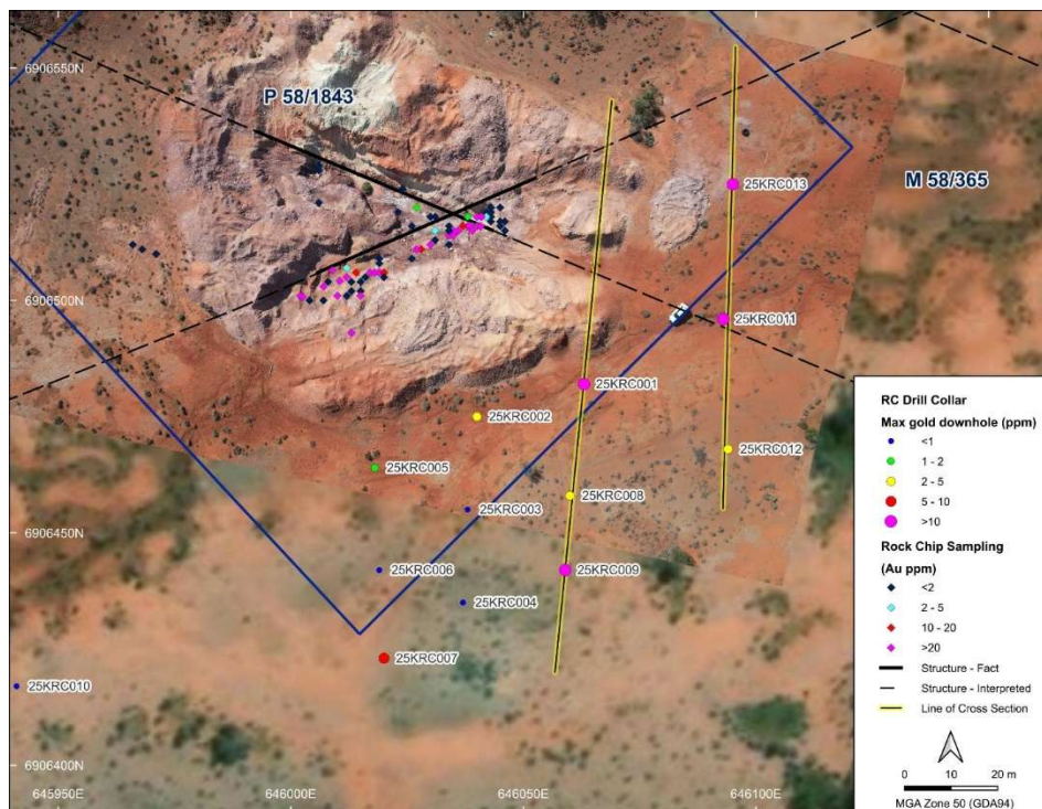
Figure 2: RC Drillhole Location Plan, Killarney Project
