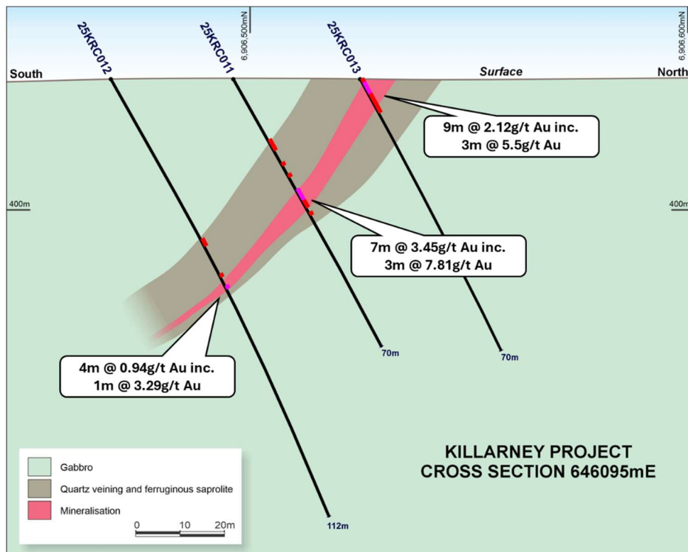
Figure 4: Cross Section 646095E, Killarney Project
