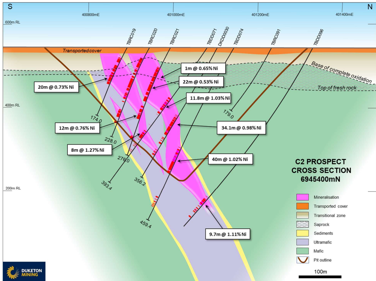
Figure 14: C2 Cross Section
