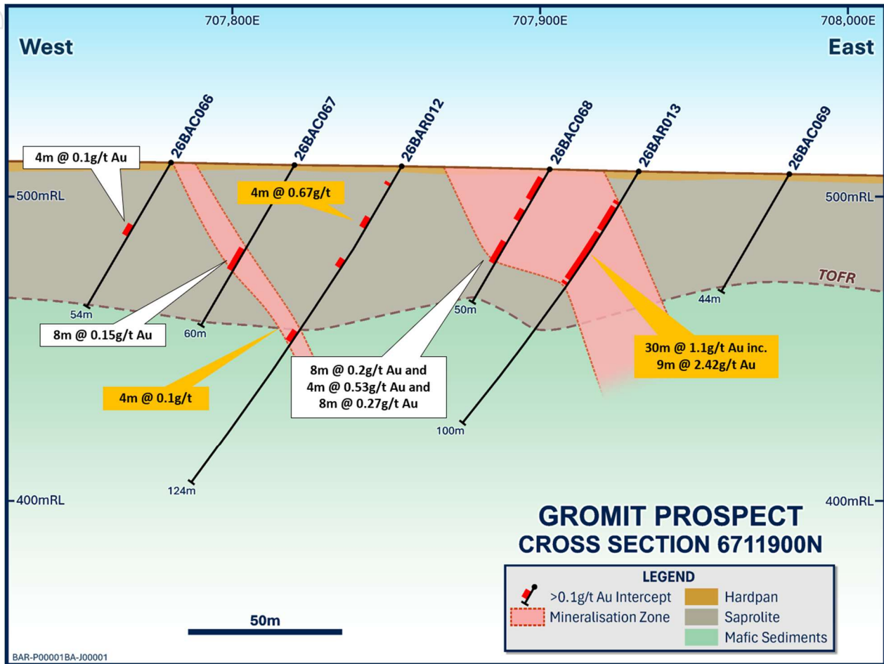
Figure 7: Gromit Prospect Cross Section 6711900N
