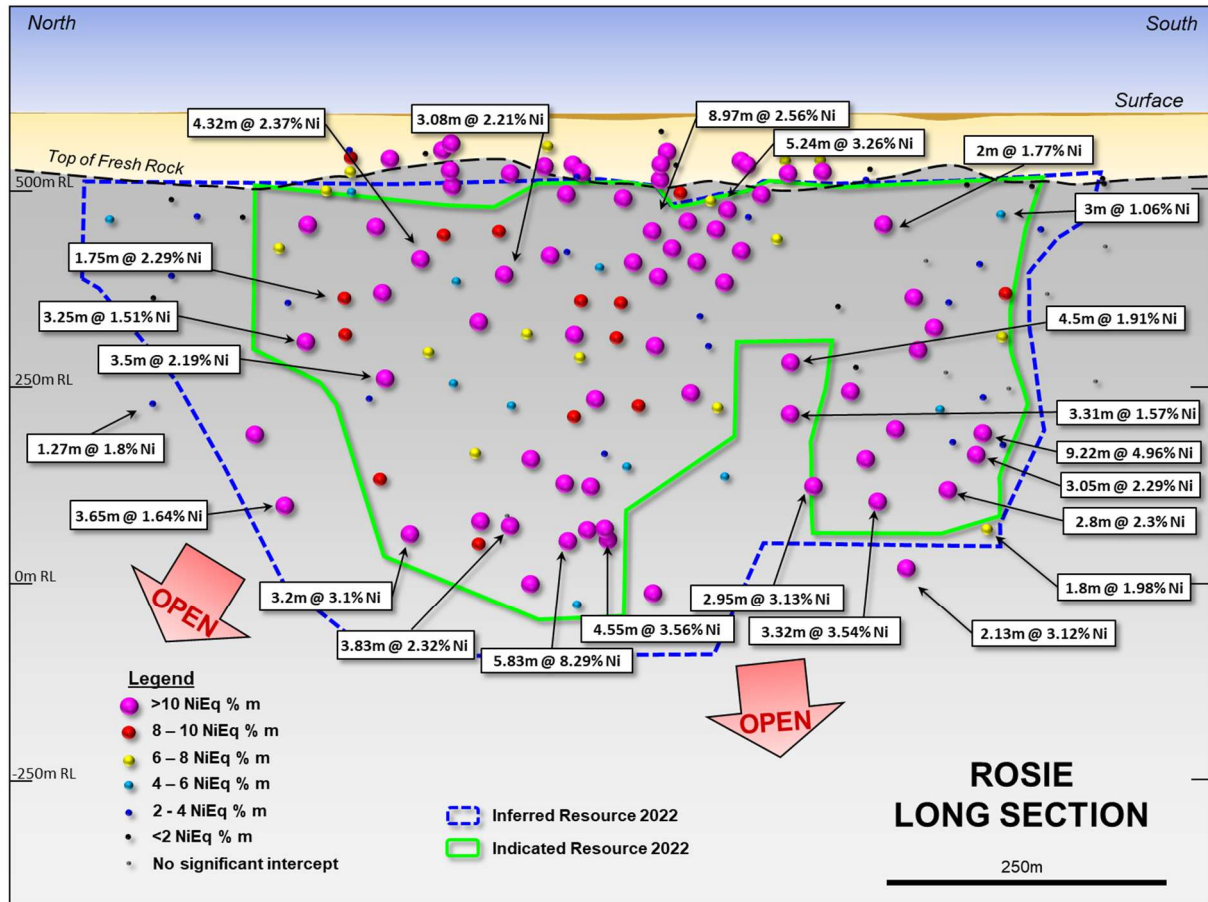
Figure 13: Long section of Rosie looking toward the northeast showing significant intercepts
