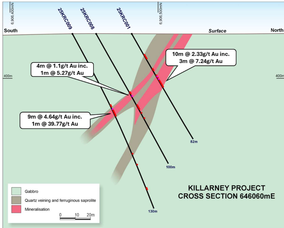
Figure 3: Cross Section 646060E, Killarney Project
