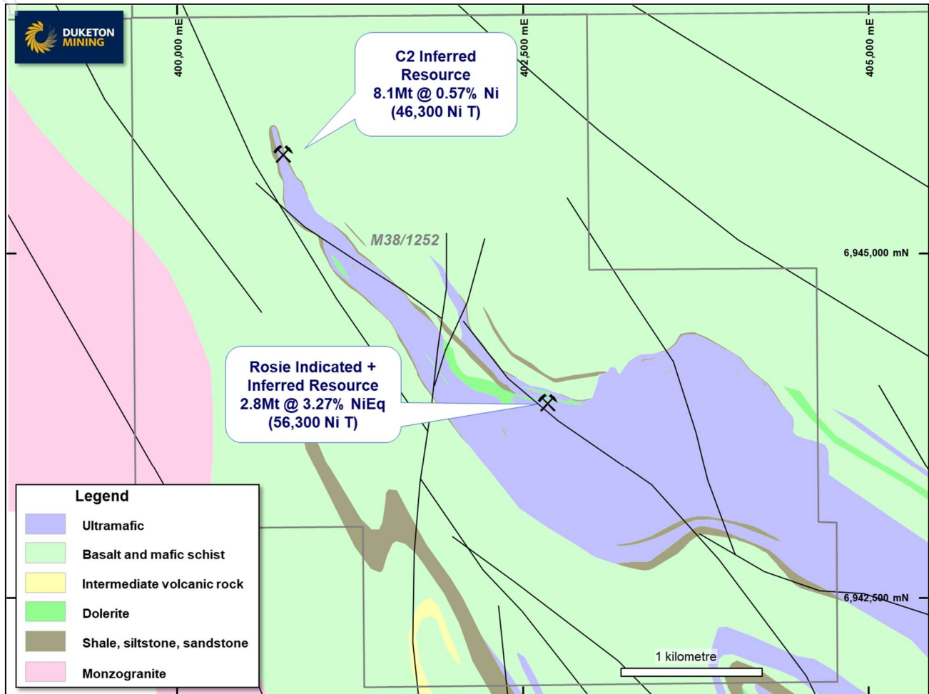
Figure 12: Location Plan of C2 and Rosie Resources.
