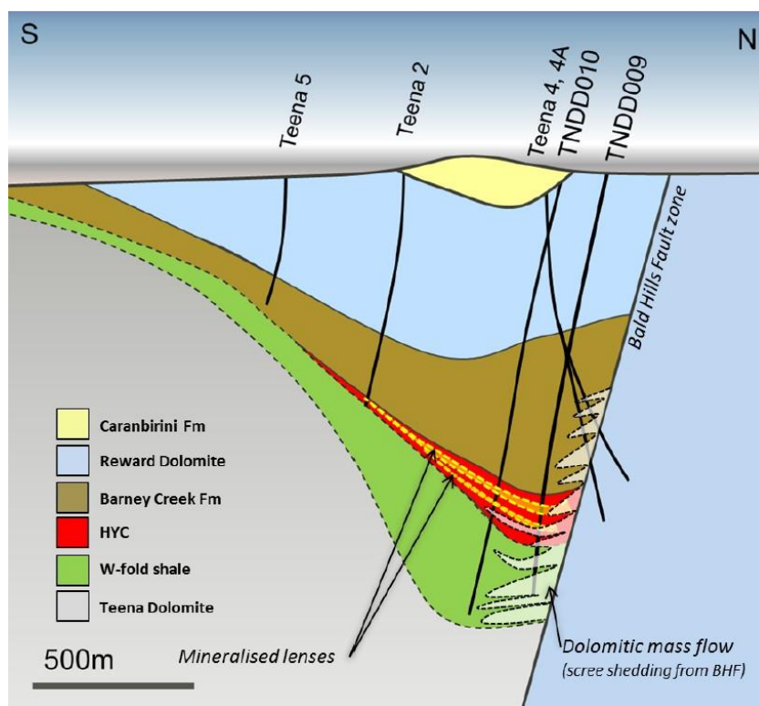
Figure 2: Schematic cross-section through the Teena deposit showing mineralisation within the Barney Creek Formation in a fault-bounded sub-basin developed along the Bald Hills Fault zone. This is a regional analogue and is not a cross-section through the Batten target.
