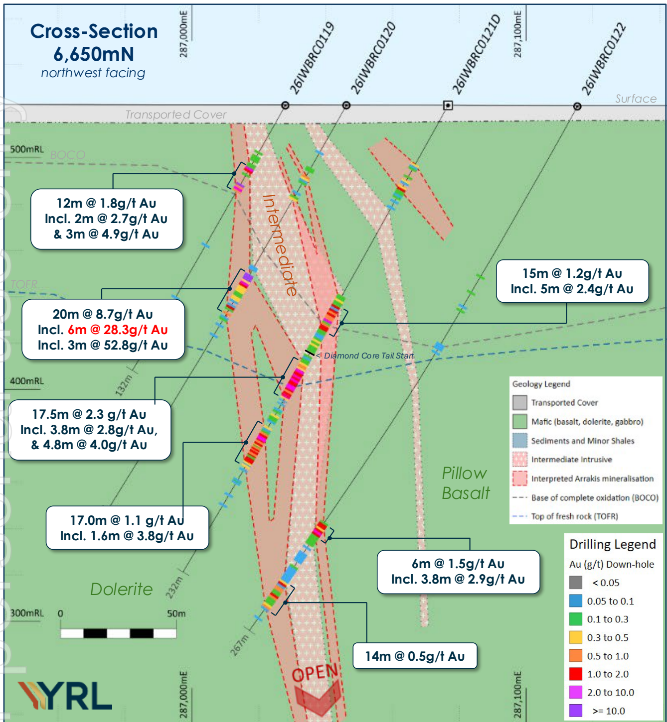
Figure 3: Arrakis 6,650mN cross-section showing all recently received drilling results, including significant intercepts from 26IWBR0120 and 26IWBR0121D. The section location is shown in Figure 5. The section shows all drilling within +/- 25m of the section plane.
