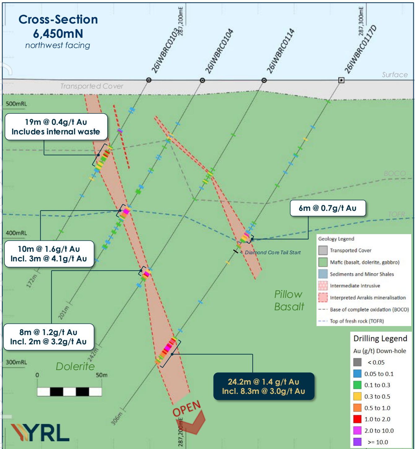
Figure 1: Arrakis 6,450mN cross-section showing all recently received drilling results, including significant intercepts from 26WBRC0117D. The section location is shown in Figure 5. The section shows all drilling within +/- 25m of the section plane.
