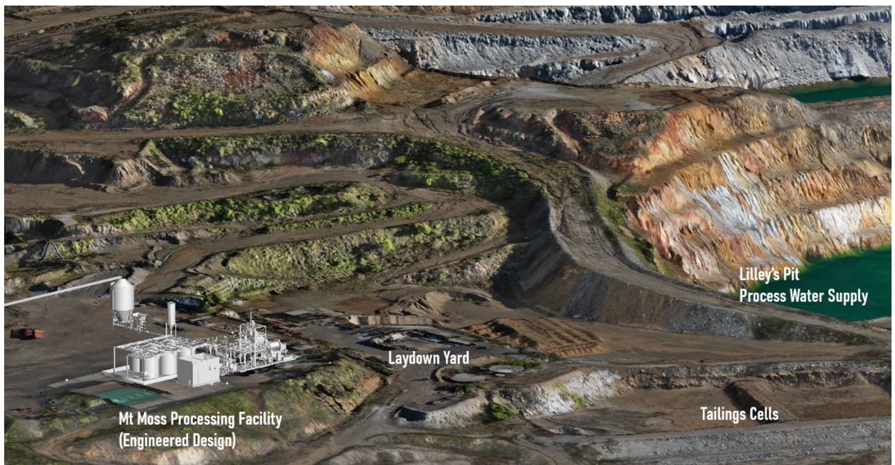
Figure 10: Designed Mt Moss Processing Facility on the site 3D model showing the location of the tailing's facility, the likely source of mill process water and the site laydown yard.
