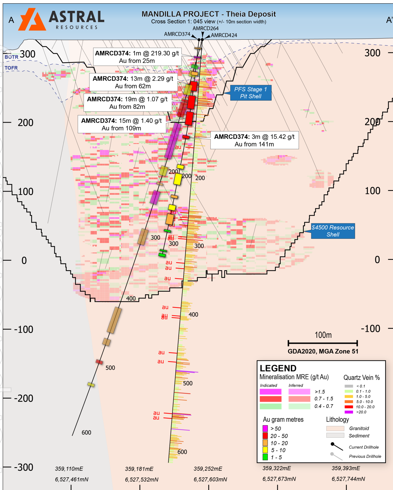
Figure 4 – Cross-section A-A' view of the Theia Deposit showing the drill trace and assay results for AMRCD374. (please note - previous drillholes are not drawn with reported assay intervals).
