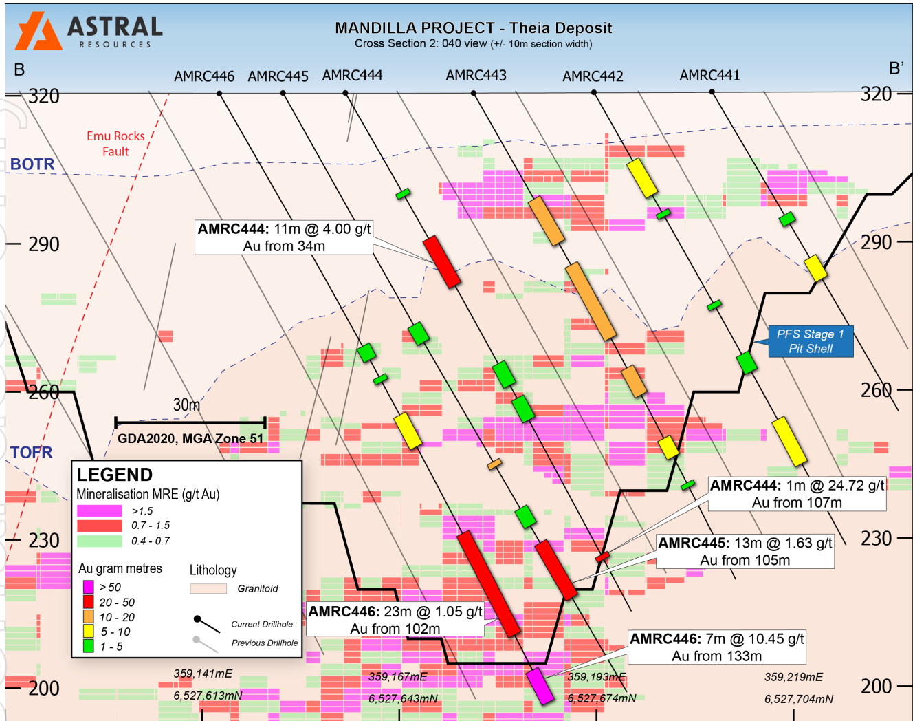
Figure 3 – Cross-section B-B' view of the Theia Deposit showing the drill trace and assay results for the current in-fill RC drilling (please note - previous drillholes are not drawn with reported assay intervals).
