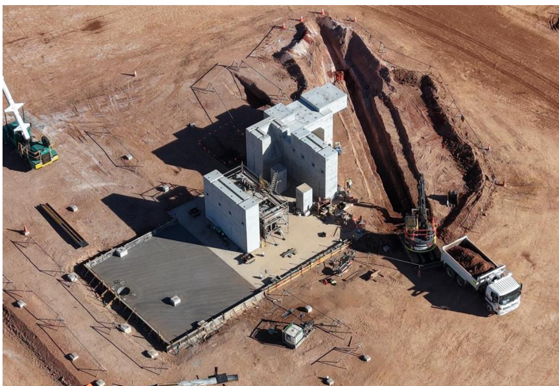
Figure 3: Grinding and Classification area – major concrete foundations complete
