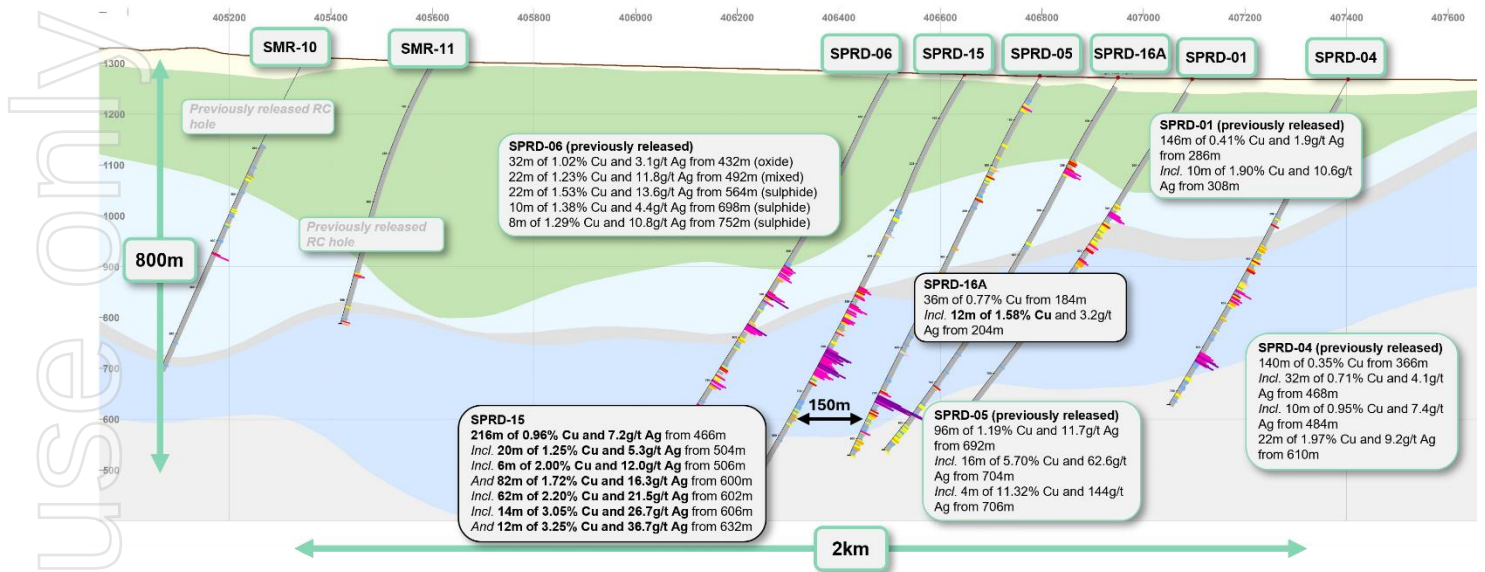
Figure 5: Cross Section Looking North – Pampa Medina 7,440,950 N
