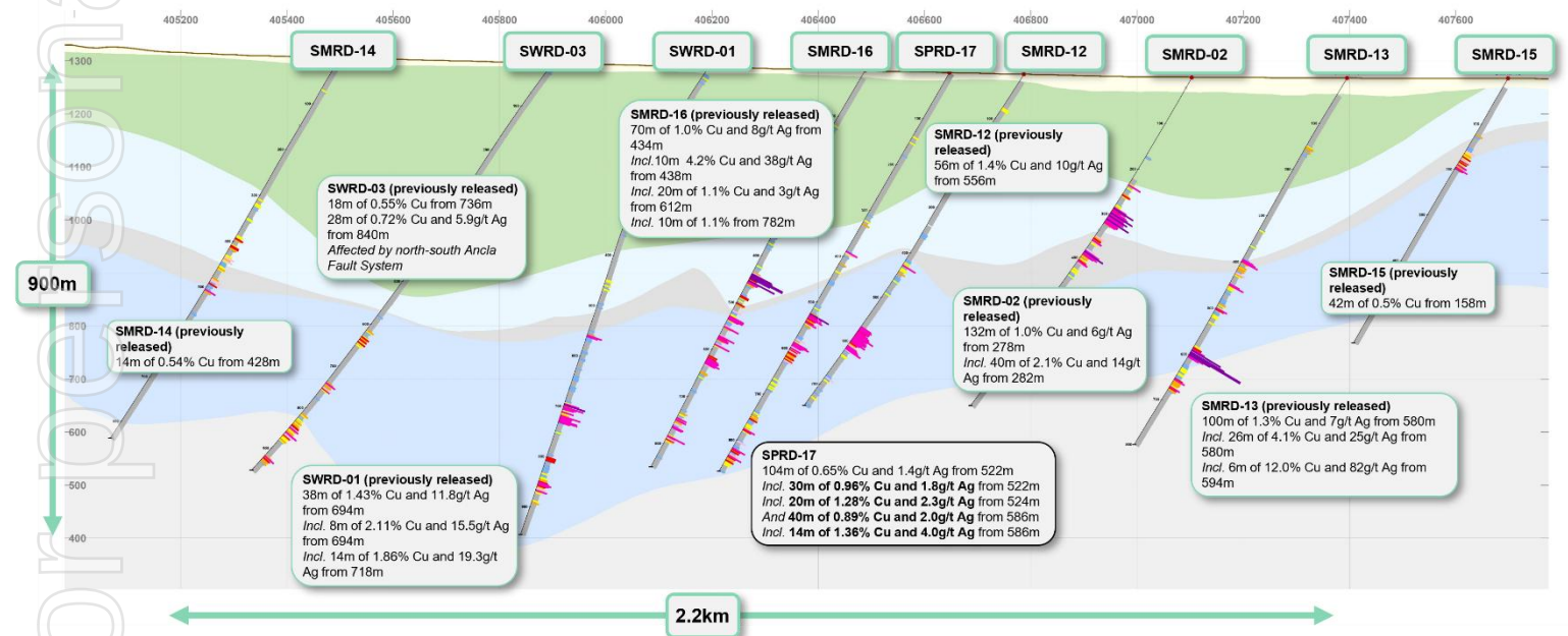
Figure 6: Cross Section Looking North – Pampa Medina 7,440,800 N
