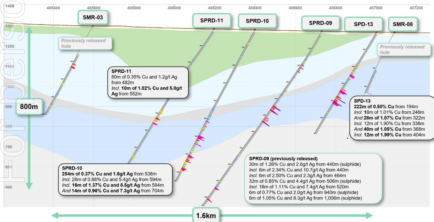
Figure 8: Cross Section Looking North – Pampa Medina 7,440,350 N
