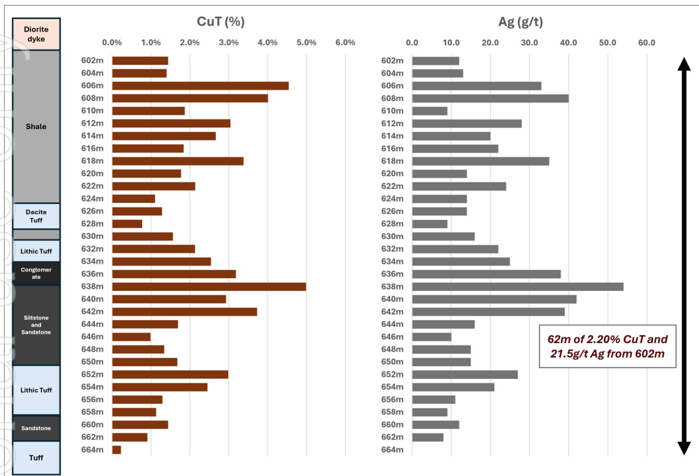
Figure 4: Downhole Lithology and Mineralized Intersection – SPRD-15 from 602m Downhole
