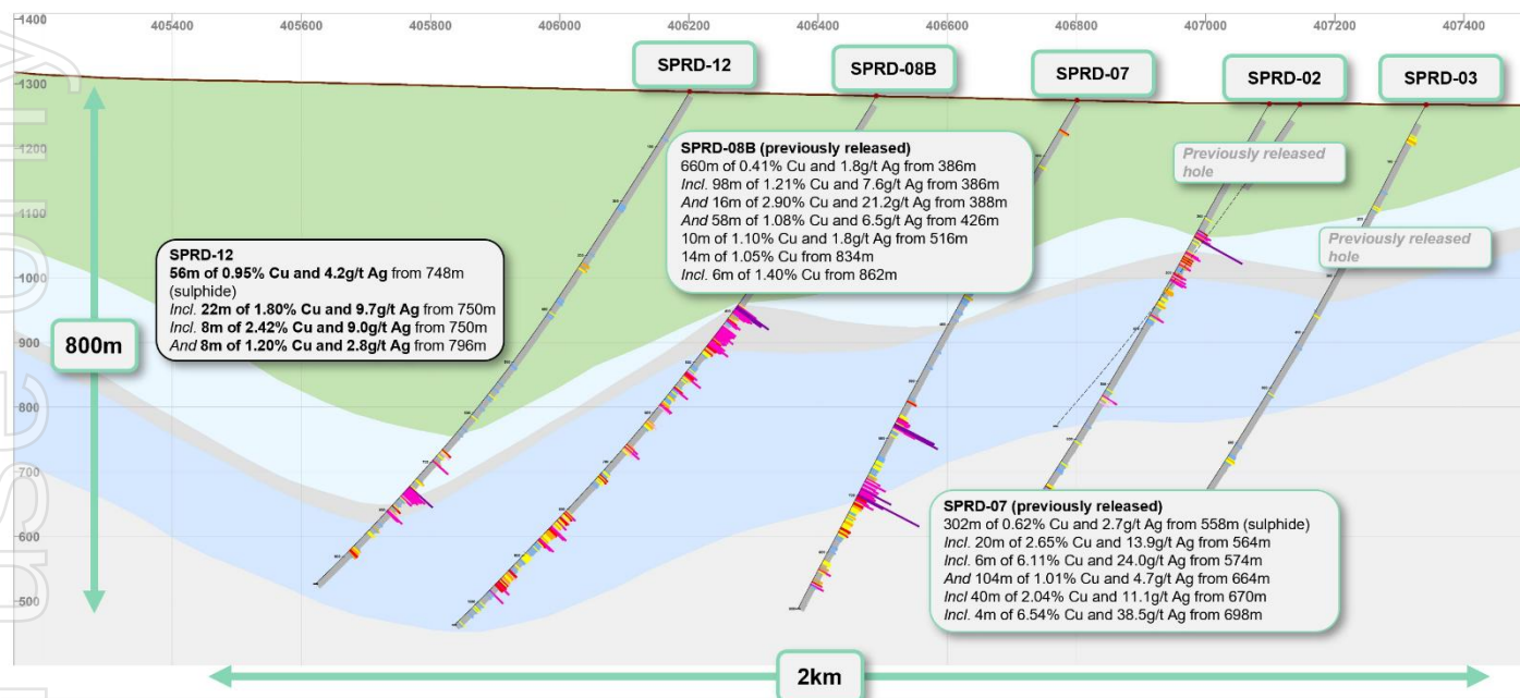
Figure 7: Cross Section Looking North – Pampa Medina 7,440,650 N
