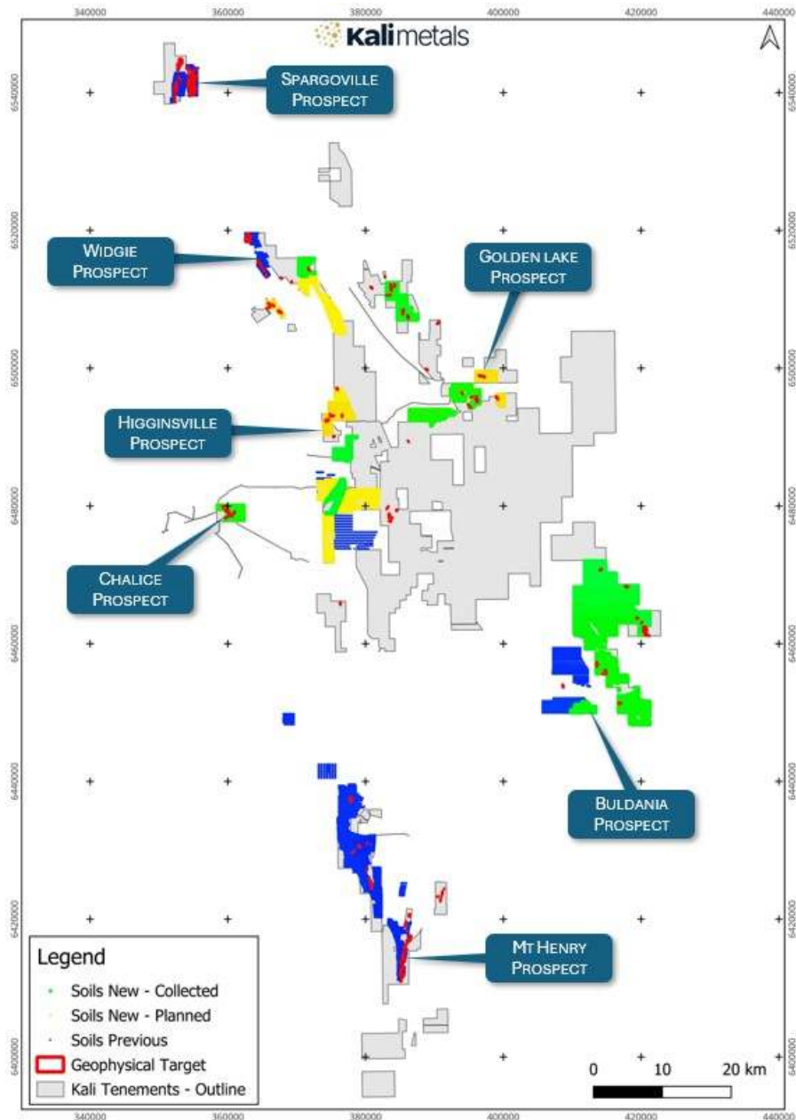
Figure 10 – Higginsville Lithium Project soils program locations
