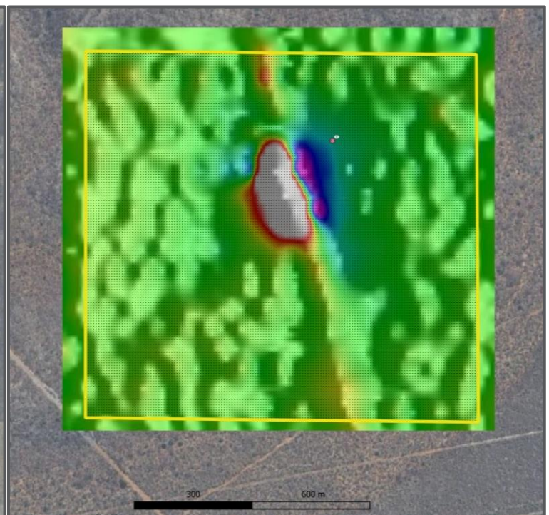
Figure 7. Abenab magnetic anomaly
