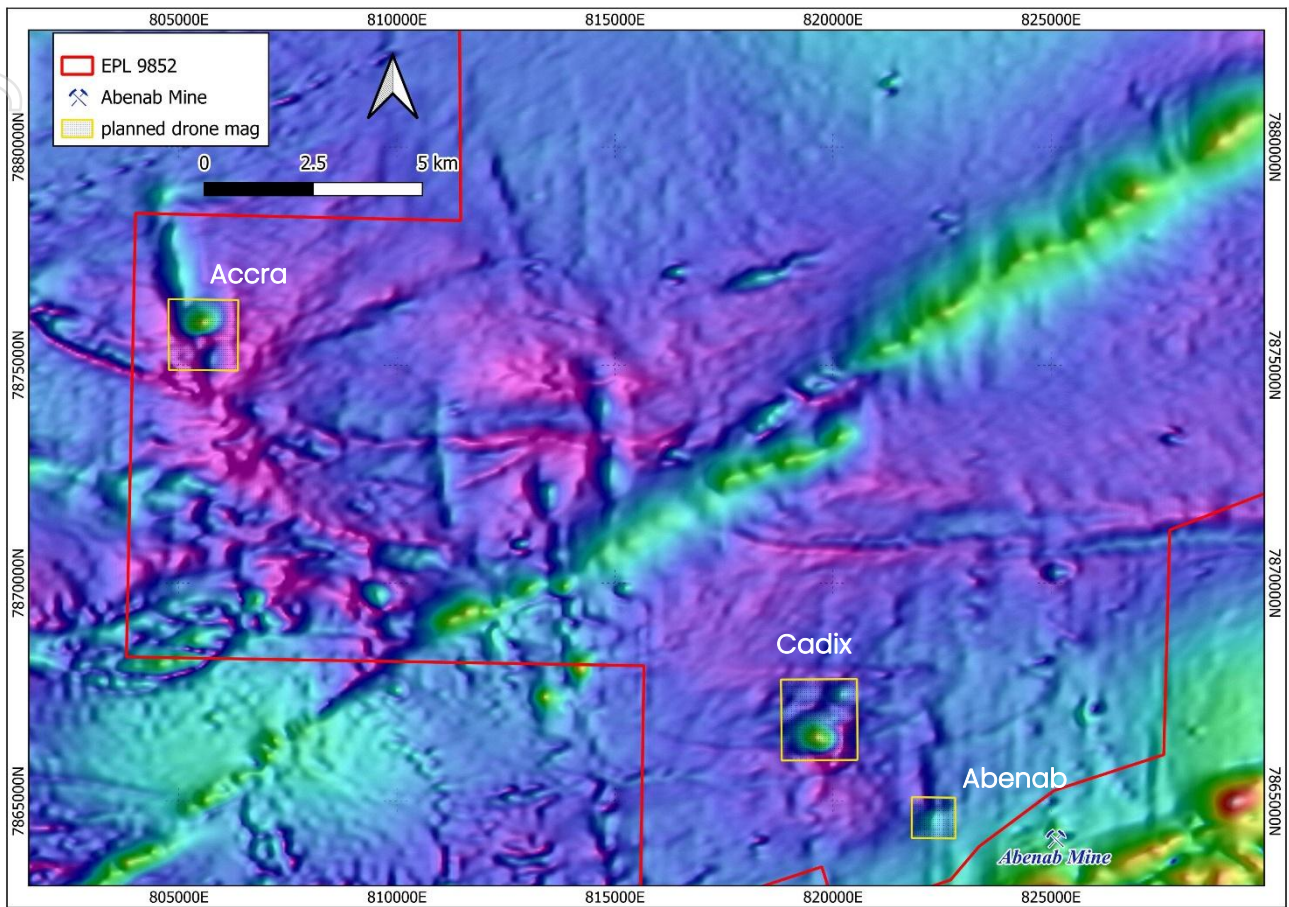
Figure 5. Drone magnetic survey blocks.
