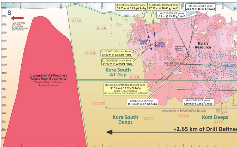
Kainantu Cross Section
