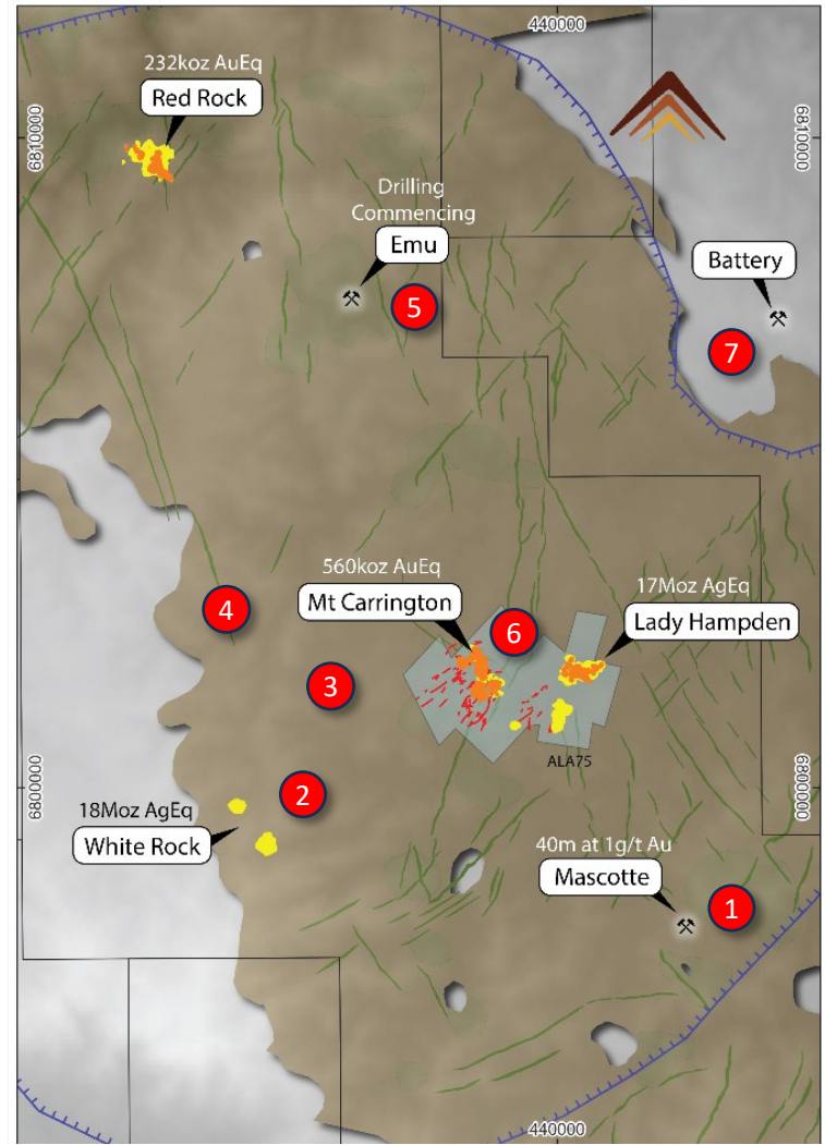
Mt Carrington regional geology plan view showing Major Prospects and known mineralisation projected to surface (yellow) and gold dominant mineralisation (orange) over the Drake Volcanics and historical mapped mineralised veins (red)
