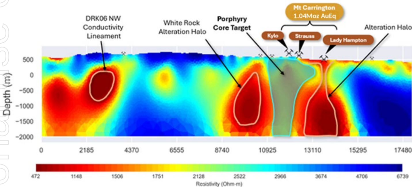
MT Resistivity across the Mt Carrington Deposits and White Rock Alteration Halo 1
