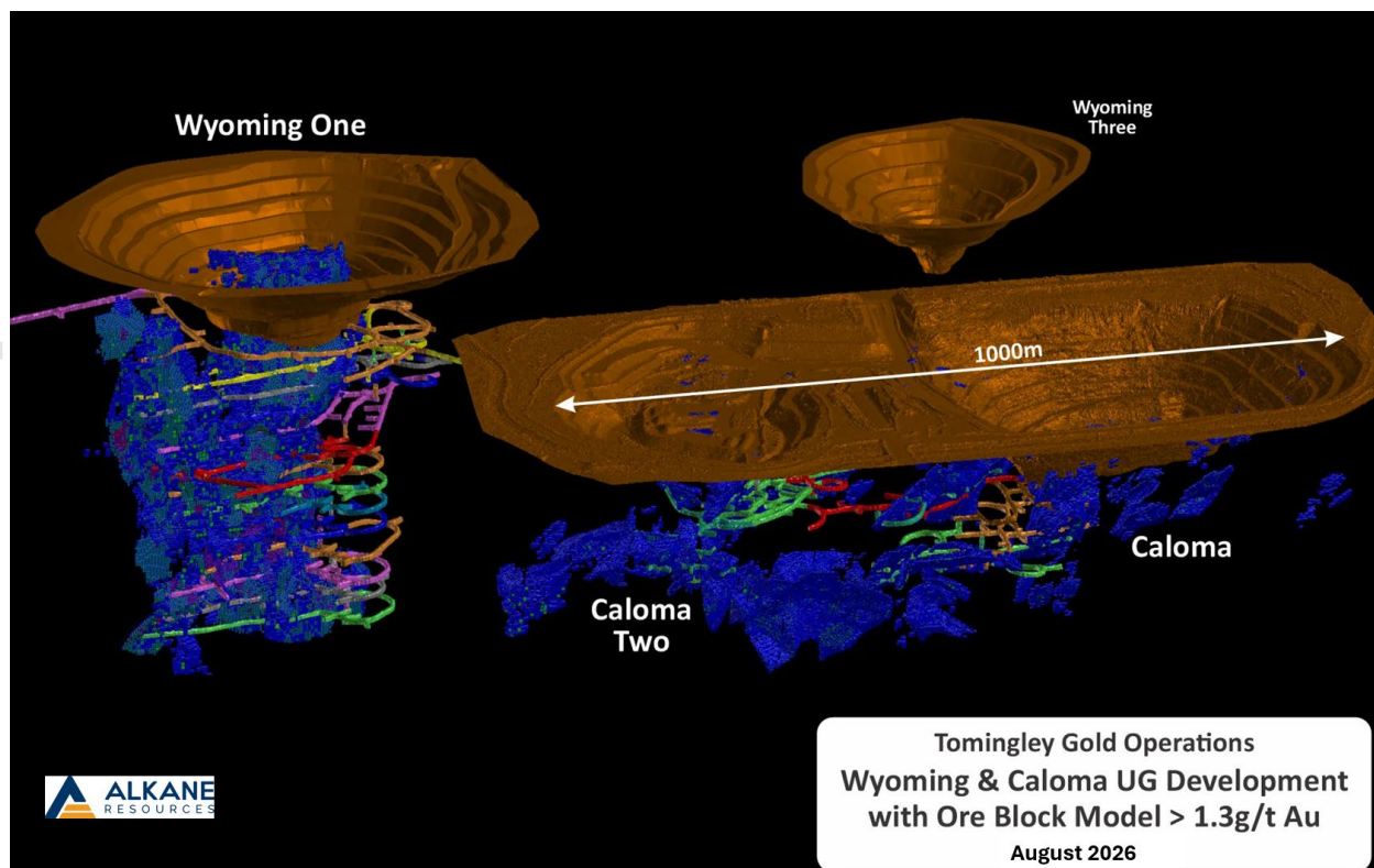
Figure 3. Isometric view of the Wyoming and Caloma block models with current pit shapes and underground development.
