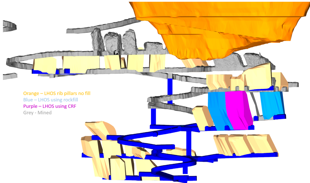
Figure 4: Isometric View of Caloma One Pit and Stope Shapes
