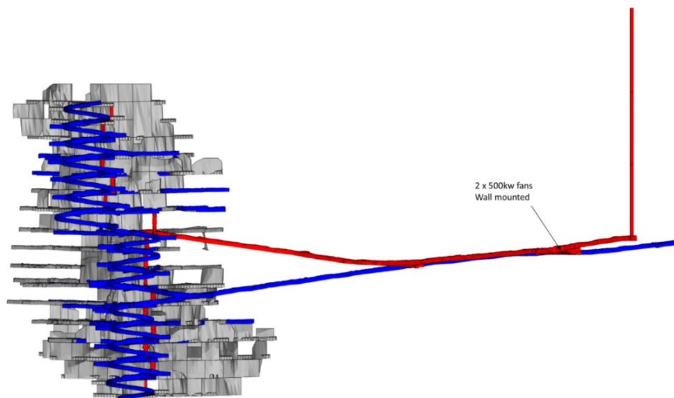
Figure 7: Primary Ventilation for Roswell (TGEF – Reserves Only)
