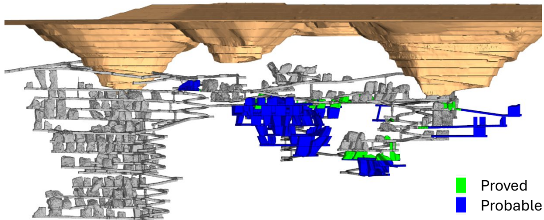
Figure 8: Isometric view of Caloma One and Caloma Two Life-of-Mine design by Ore Reserve classification
