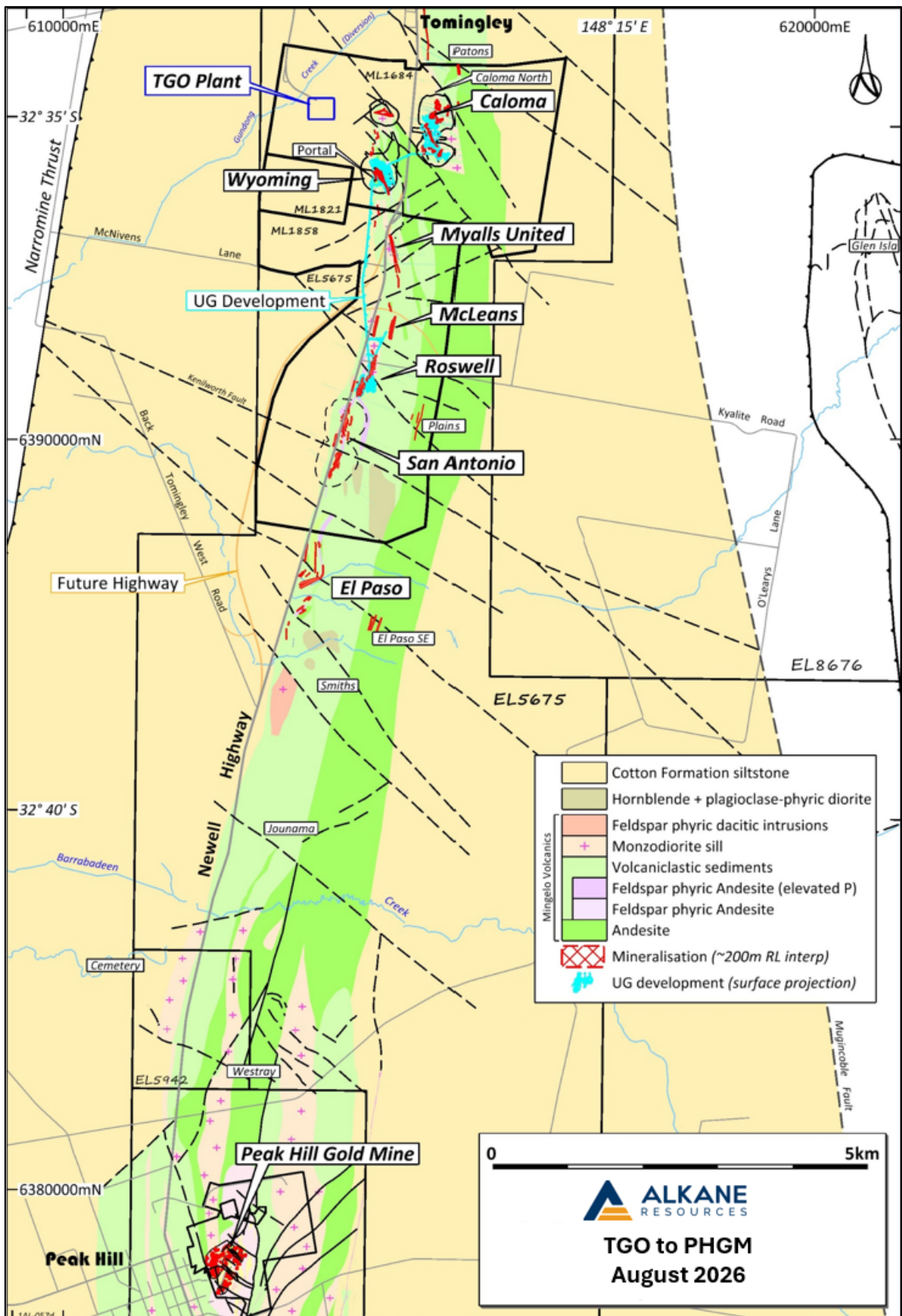
Figure 1. Geological map showing the location of mineral deposits between the Peak Hill gold mine and the Tomingley Gold Mine
