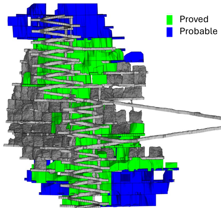
Figure 9: Isometric view of Roswell Life-of-Mine design by Ore Reserve classification
