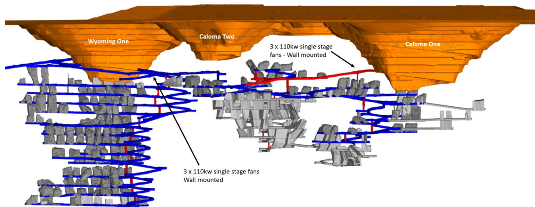
Figure 6: Primary Ventilation for Wyoming One, Caloma One and Caloma Two
