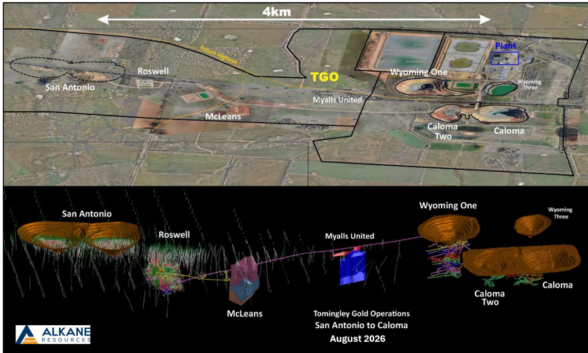
Figure 10: Perspective view of the as built and planned development at Tomingley Gold Operation
