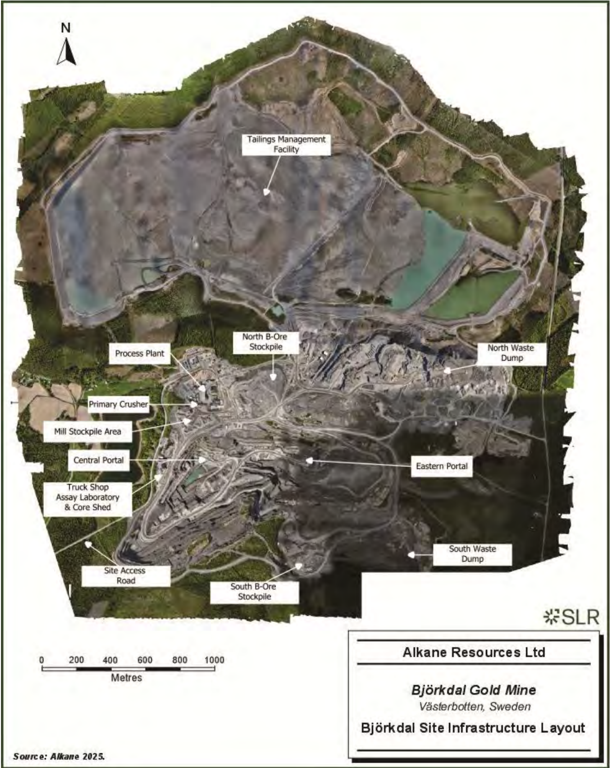
Figure 18-1: Björkdal Site Infrastructure Layout
