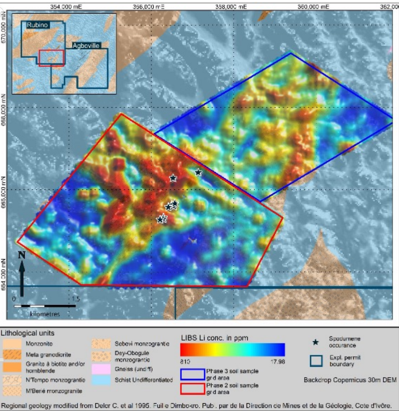
Figure 2: Consolidated Rubino Phase 2 and Phase 3 Li (ppm) in soil grid results with spodumene pegmatite discovery sites.
