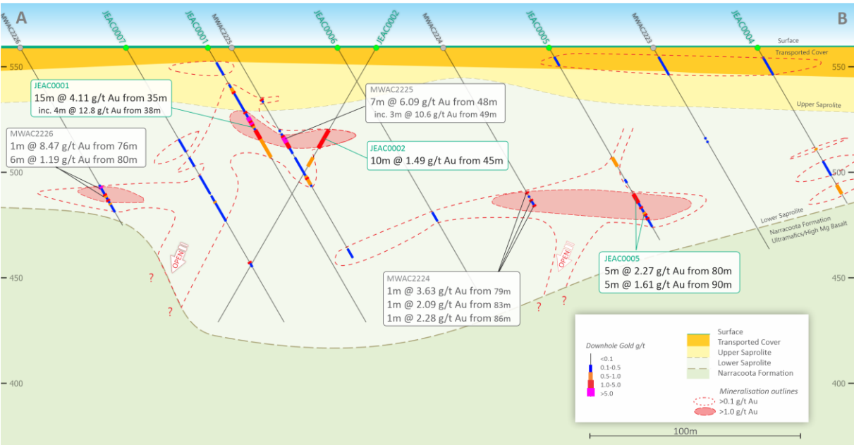
Figure 2. Drilling Cross Section – Jacques East Prospect
