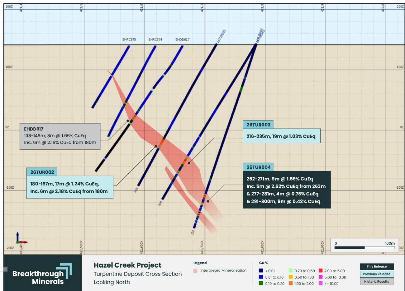
Figure 3: 26TUR004 cross section showing drill intersections and interpreted mineralisation.
