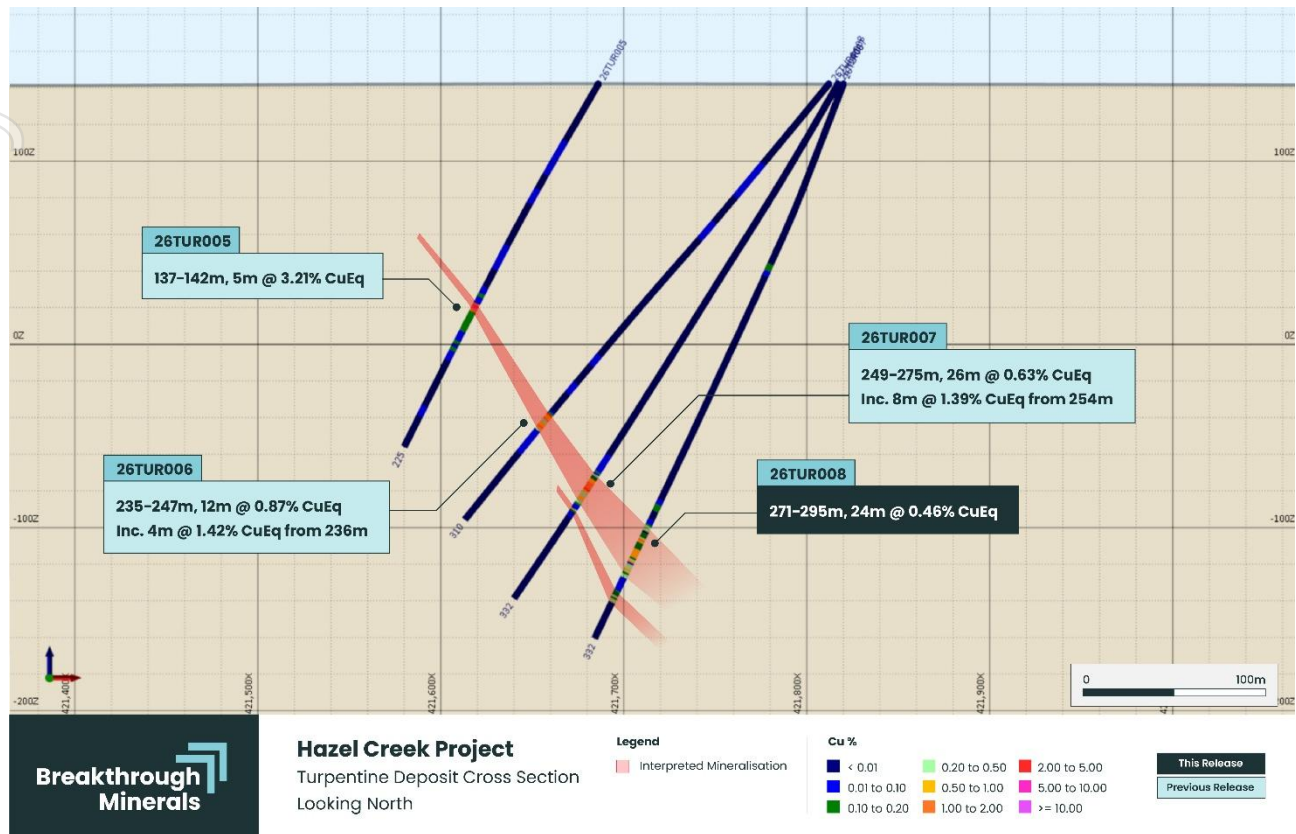
Figure 4: 26TUR008 cross section showing drill intersections and interpreted mineralisation outside the Turpentine Mineral Resource model
