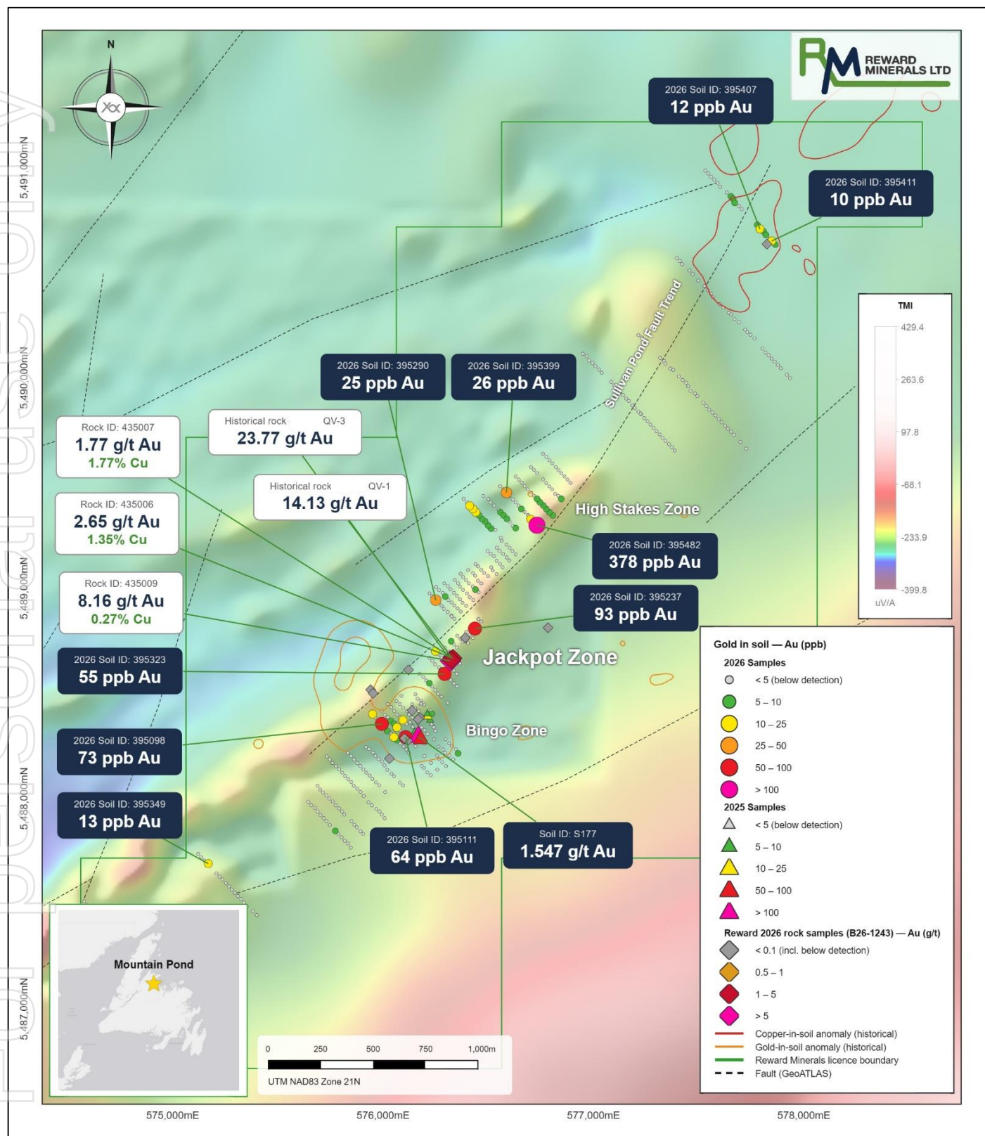
Figure 2 – Mountain Pond Project total magnetic intensity image, the interpreted position of the Sullivan Pond Fault Trend, previously released rock and soil results where marked, and new soil sample results for gold only. The multi-element ICP-34 analysis for the new soil samples will be released once all results are received and collated.
