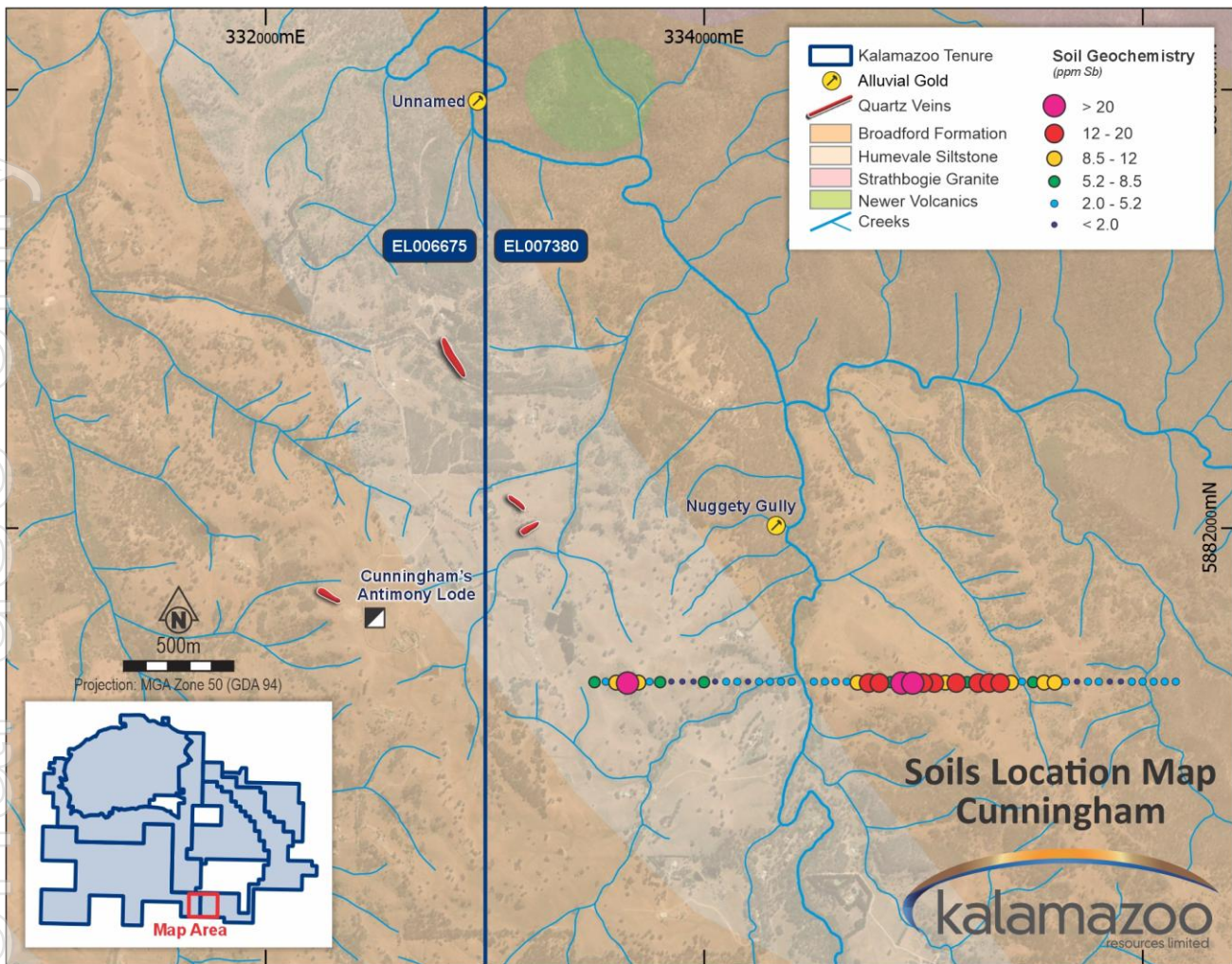
Figure 5. Mapped quartz veining, alluvial gold workings, hard rock gold and antimony workings and recent antimony soil results from Cunningham's Prospect
