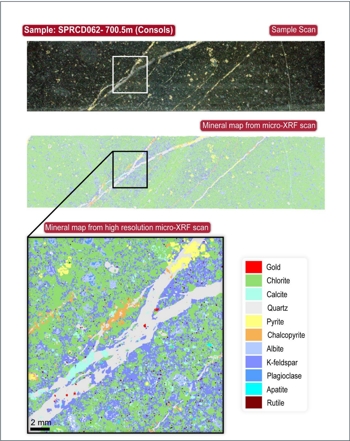
Figure 5: An example to show results of micro-XRF scanning with an AMICS (Advanced Mineral Identification and Characterisation System) generated mineral map on half core. The whole sample surface was mapped using a 100 µm per pixel resolution with a follow up area of approximately 20 mm x 20 mm scanned at 20 µm per pixel. Twenty-six gold grains between 20 and 412 µm in size were detected in the high-resolution scan. The gold grains largely occur within or adjacent to a quartz-pyrite-K-feldspar-chalcopyrite vein with K-feldspar alteration halo.
