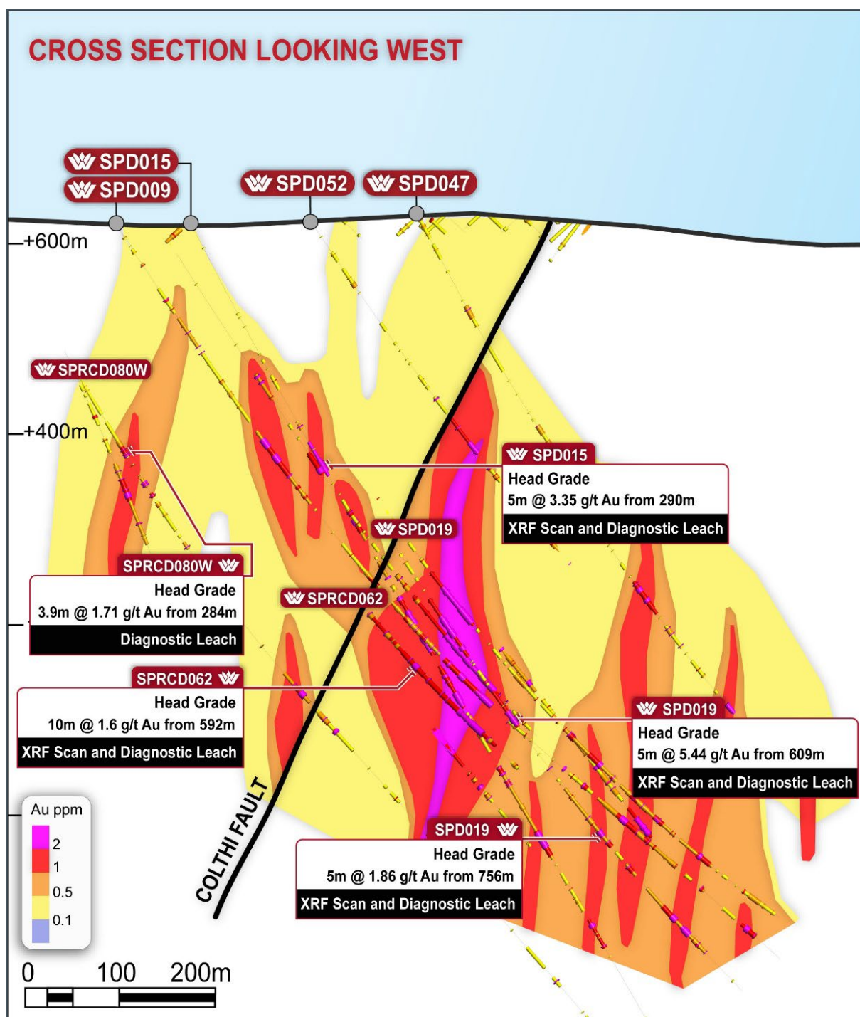
Figure 2: Consols Zone cross section showing sample locations (SPD011 off section)
