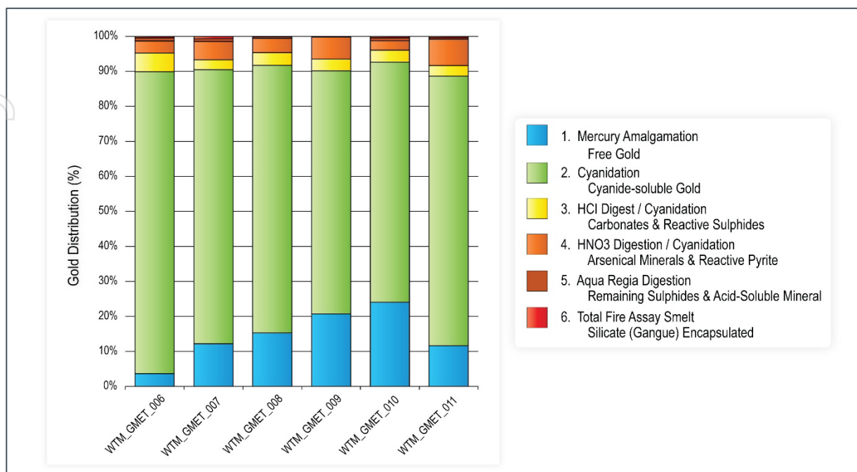
Figure 6: Results of diagnostic leach and gravity recovery tests for gold deportment on bulk (10 kg) core samples indicate that >89% of gold may be recovered through a combination of gravity and cyanide leach.
