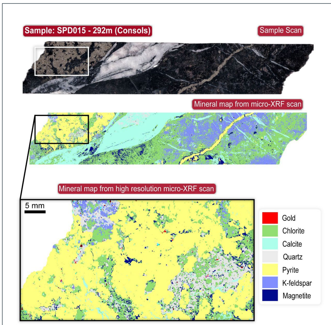
Figure 4: An example to show results of micro-XRF scanning with an AMICS (Advanced Mineral Identification and Characterisation System) generated mineral map on half core. The whole sample surface was mapped using a 100 \mu\text{m} per pixel resolution with a follow up area of approximately 20 mm x 20 mm scanned at 20 \mu\text{m} per pixel. Thirty gold grains between 20 and 301 \mu\text{m} in size were detected in the high-resolution scan. The gold grains largely occur in locations interstitial to pyrite with quartz and chlorite.
