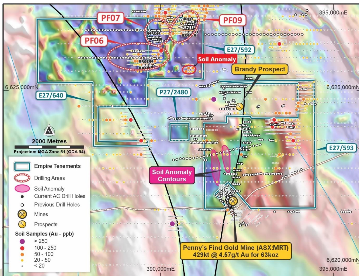
Figure 1. Pennys Gold Project Soil Anomalies
