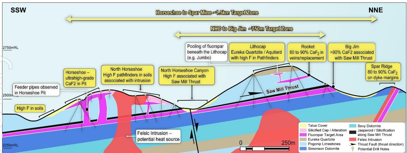
Figure 2 Schematic cross-section from Horseshoe to Big Jim/Spar, with preliminary drill designs
