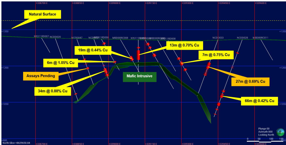
Figure 2. Nyungu Central drilling section at 8629650mN showing recent NCDD033 drilling result (looking north)
