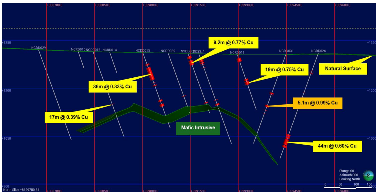
Figure 3. Nyungu Central drilling section at 8629750mN showing recent NCDD031 drilling result (looking north)
