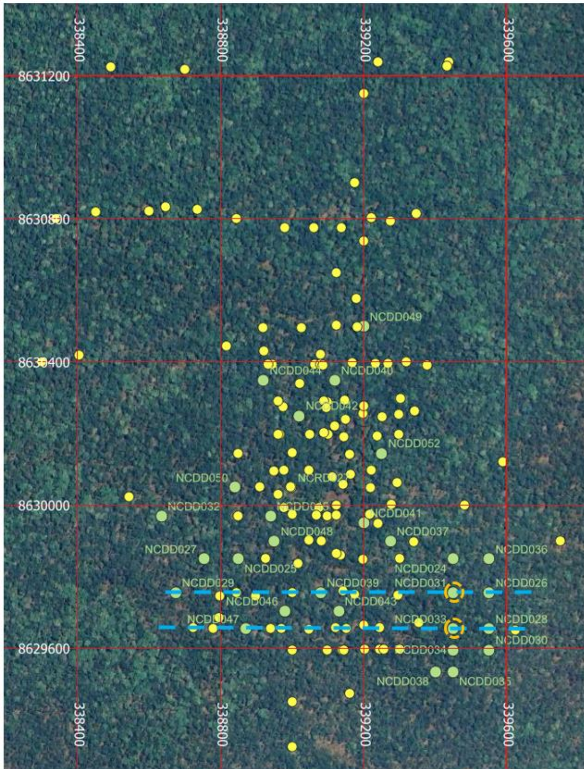
Figure 1. Nyungu Central drill hole collar plan showing Phase 3 drill holes (green); pre-2026 holes (yellow); reported holes (dashed orange) and cross section projections shown in Figures 2 and 3 (as dashed blue line)
