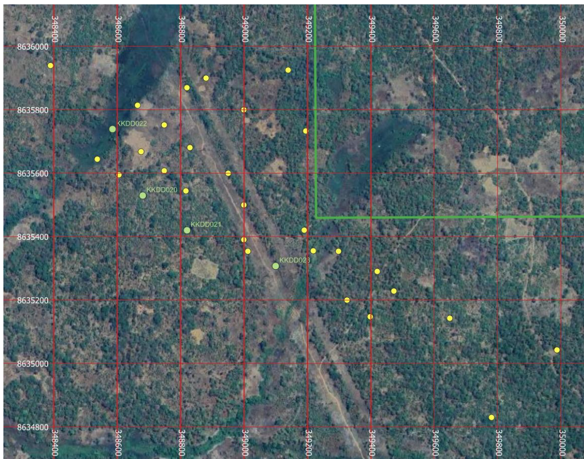
Figure 5. Kabikupa drill hole collar plan showing Prospect Phase 3 drill holes (green), pre-2026 holes (yellow)
