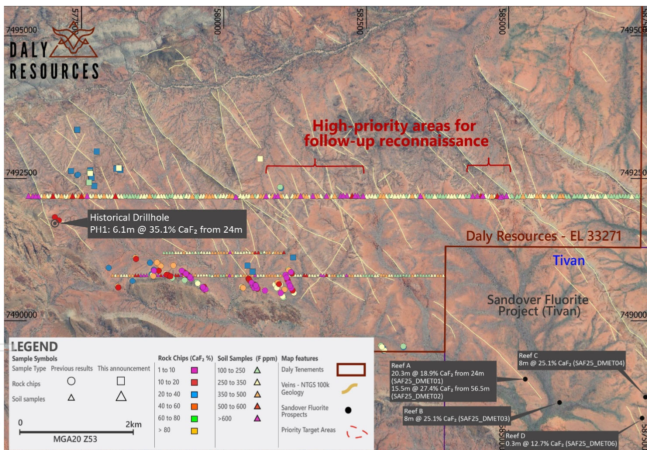
Figure 2: Map showing closer view of eastern priority target area highlighting the new fluorine-anomalous areas that require on ground follow-up. Results in the southeast are from Tivan drilling within Tivan tenure.
