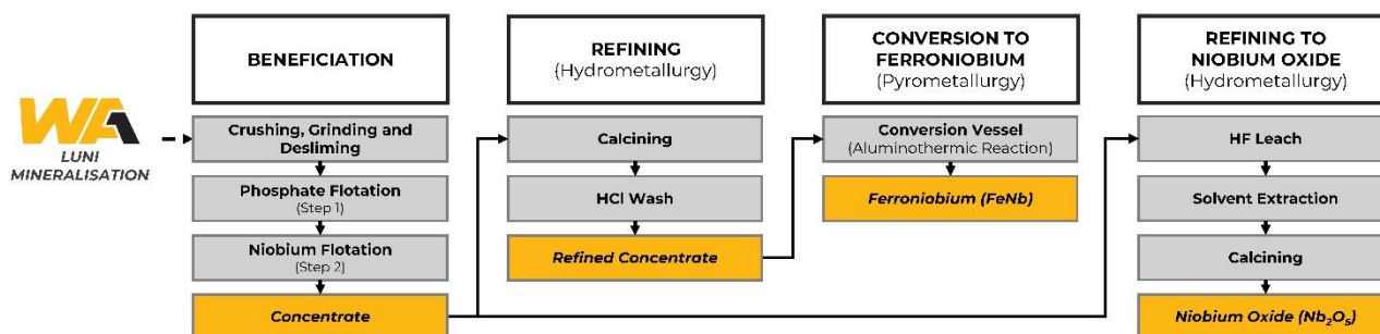
Figure 5: Simplified process flowsheet to produce proof-of-concept ferroniobium and niobium oxide
