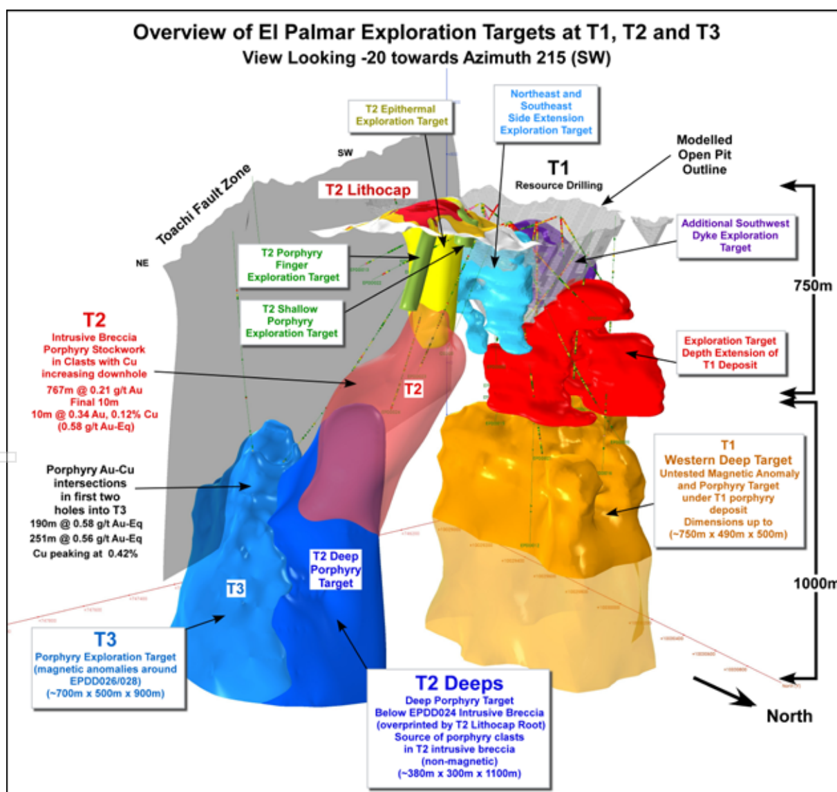
Figure 8: Overview of 9 of the 10 exploration targets defined on the El Palmar concession. View is looking at -20 degrees towards azimuth 215°.
