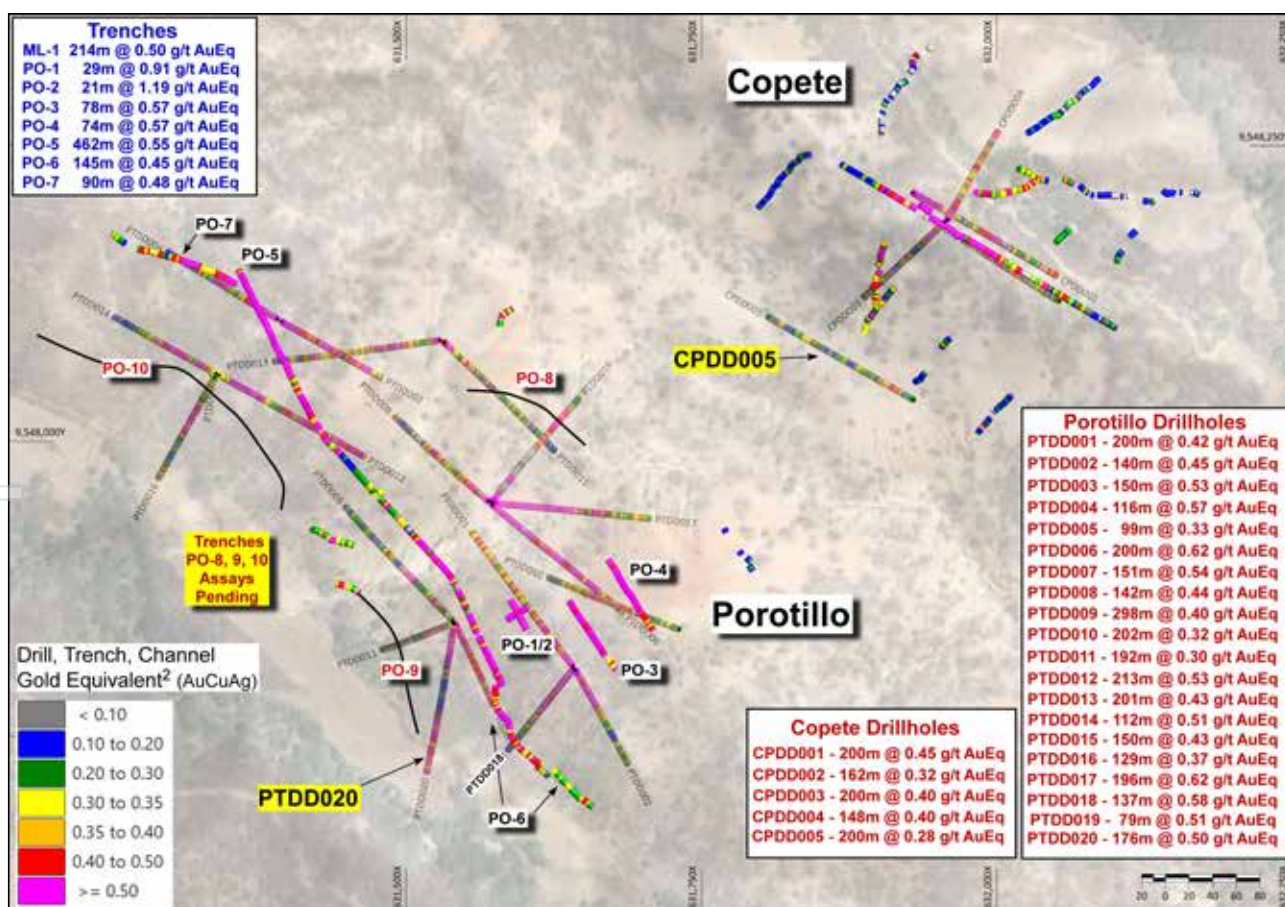
Figure 3: Drill holes and trenching results from exploration program at Porotillo and Copete conducted to 30 June 2026.
