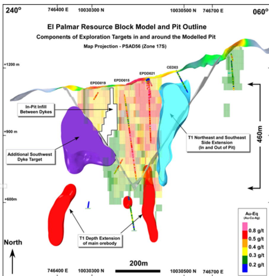
Figure 7: El Palmar T1 resource block model for grades >0.2 g/t Au-Eq and pit outline along a 240-060o cross-section and showing the exploration targets which are located within, on the sides, and immediately below the modelled T1 open pit.
