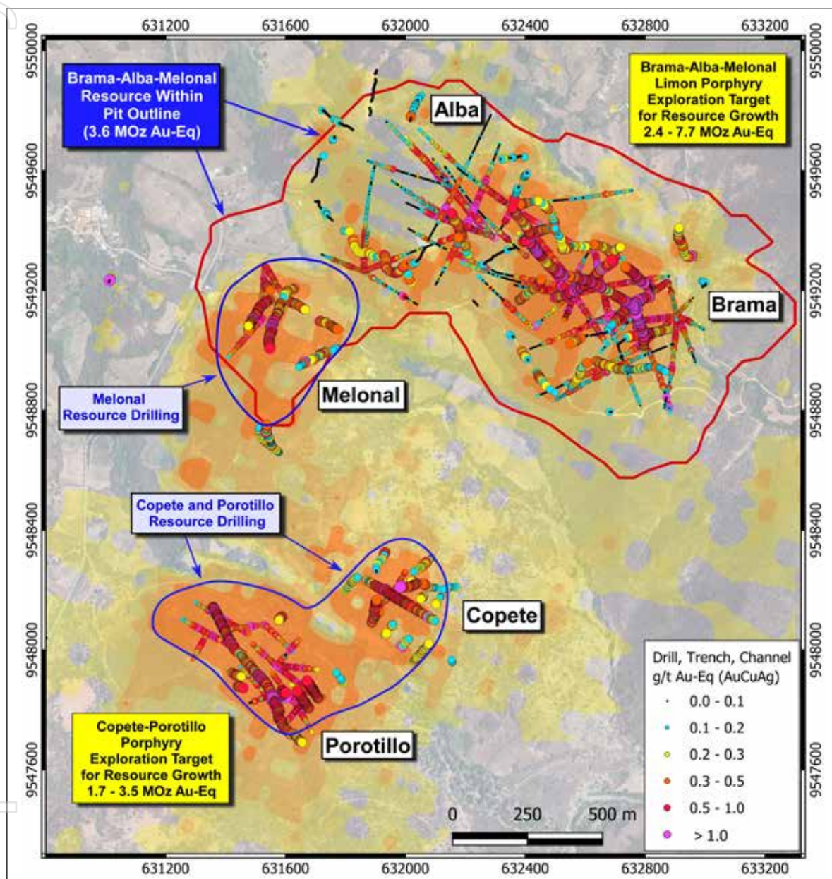
Figure 4: The cluster of five porphyry gold-copper systems in the Bramaderos concessions (Brama, Alba, Melonal, Copete and Porotillo), showing the area where resource drilling in the recent drill program was undertaken at Porotillo, Copete and Melonal to grow the Bramaderos Mineral Resource. Background colour shading is gold in soils.
