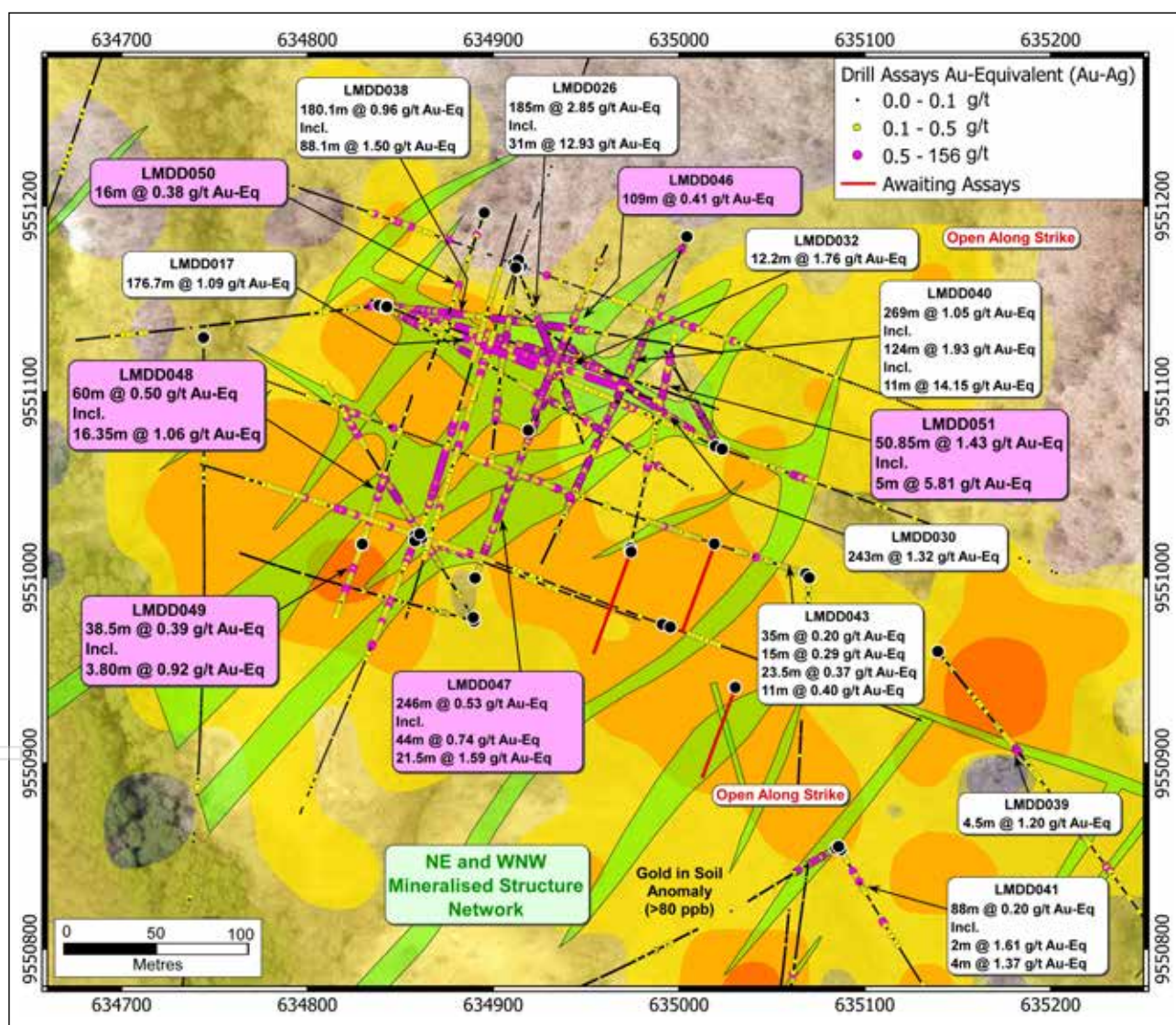
Figure 5: The Limon epithermal gold-silver system in plan view, showing multiple mineralised structures in green. High-grade domains are at intersections of NE- and WNW-trending structures. Recent intersections in holes LMDD048-051 extend mineralisation on the western and eastern sides of the Limon epithermal system. Several additional targets have been defined based on gold-in-soil and zinc-in-soil anomalies, and structural interpretation.
