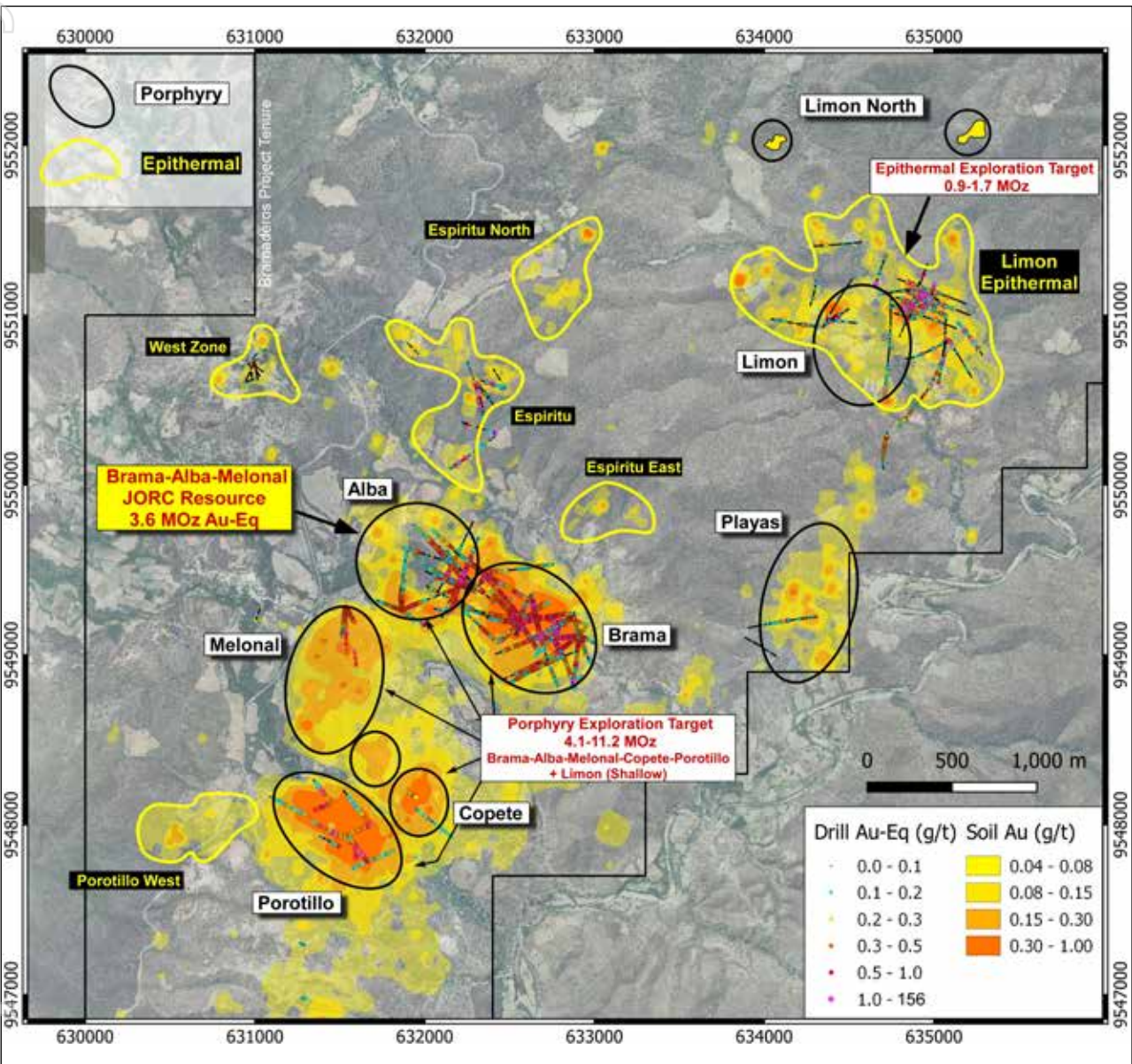
Figure 1: Overview of key prospects on the Bramaderos project, the Brama-Alba-Melonai resource area, and Exploration Target areas defined on the Bramaderos properties. The background image is gold-in-soil, highlighting the potential scale increase to be delivered with more drilling at Bramaderos across multiple targets.
