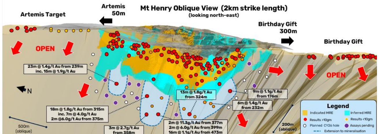
Figure 5: Mt Henry Deposit Showing Multiple Mineralised Lodges Across ~2km of Strike, With Drilling Extending Mineralisation at Depth and Along Strike. Holes with Assays Pending (purple) and Planned CY26 Drilling (white) Target Further Resource Growth, with Artemis and Birthday Gift to the Immediate North and South Providing Further Growth Opportunities.
