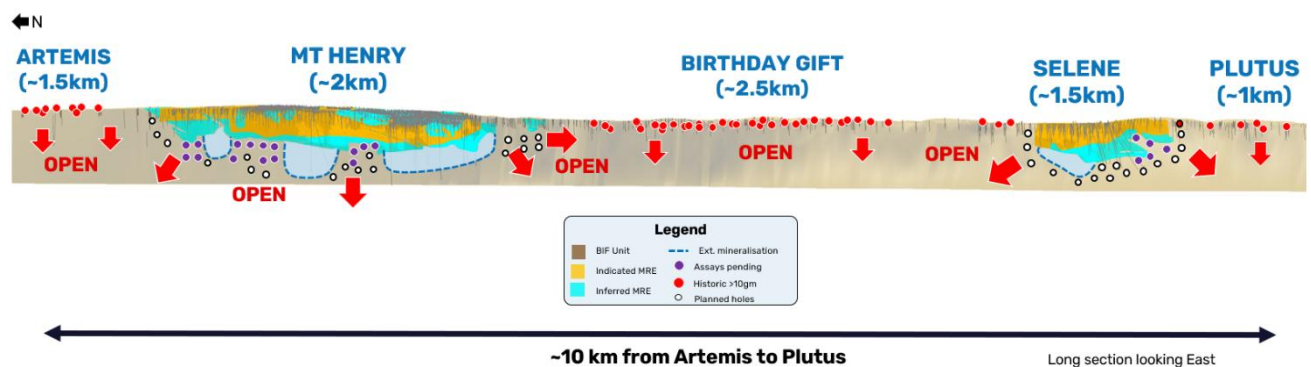
Figure 2: Current 1.8Moz Resource Boundaries at Mt Henry and Selene, Showing Recent Extensions to Gold Mineralisation Beyond the Resource, With Both Deposits Remaining Open and Ongoing Drilling Targeting Further Growth. The ~10km Mineralised Corridor from Artemis to Plutus Also Highlights the Broader Regional Growth Opportunity, Including Artemis, Birthday Gift and Plutus.
