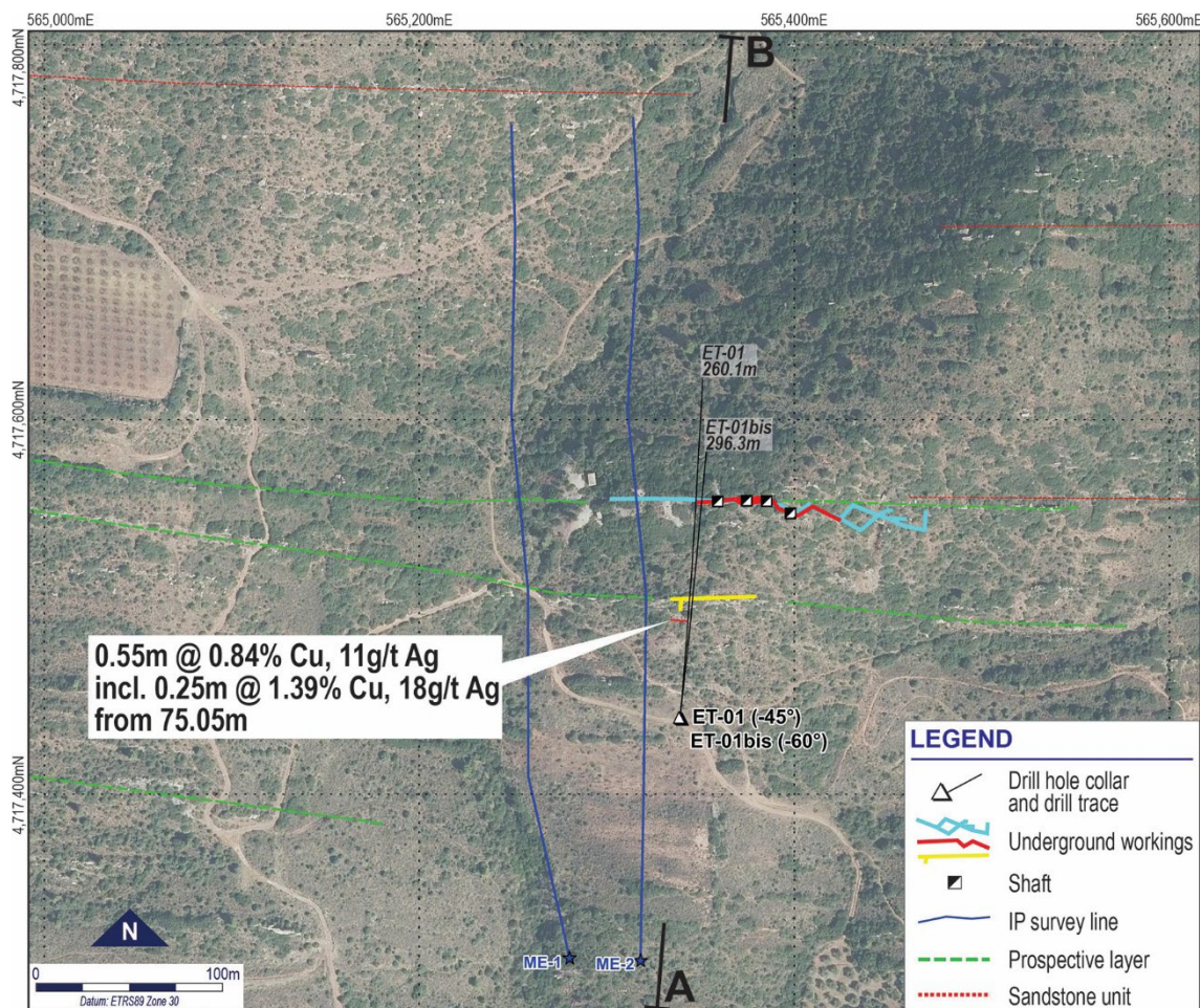
Figure 2 – Location of drill holes ET-01 and ET-01bis and Mina Emilia historical workings. Cross-section A – B (Figure 3) highlighted.
