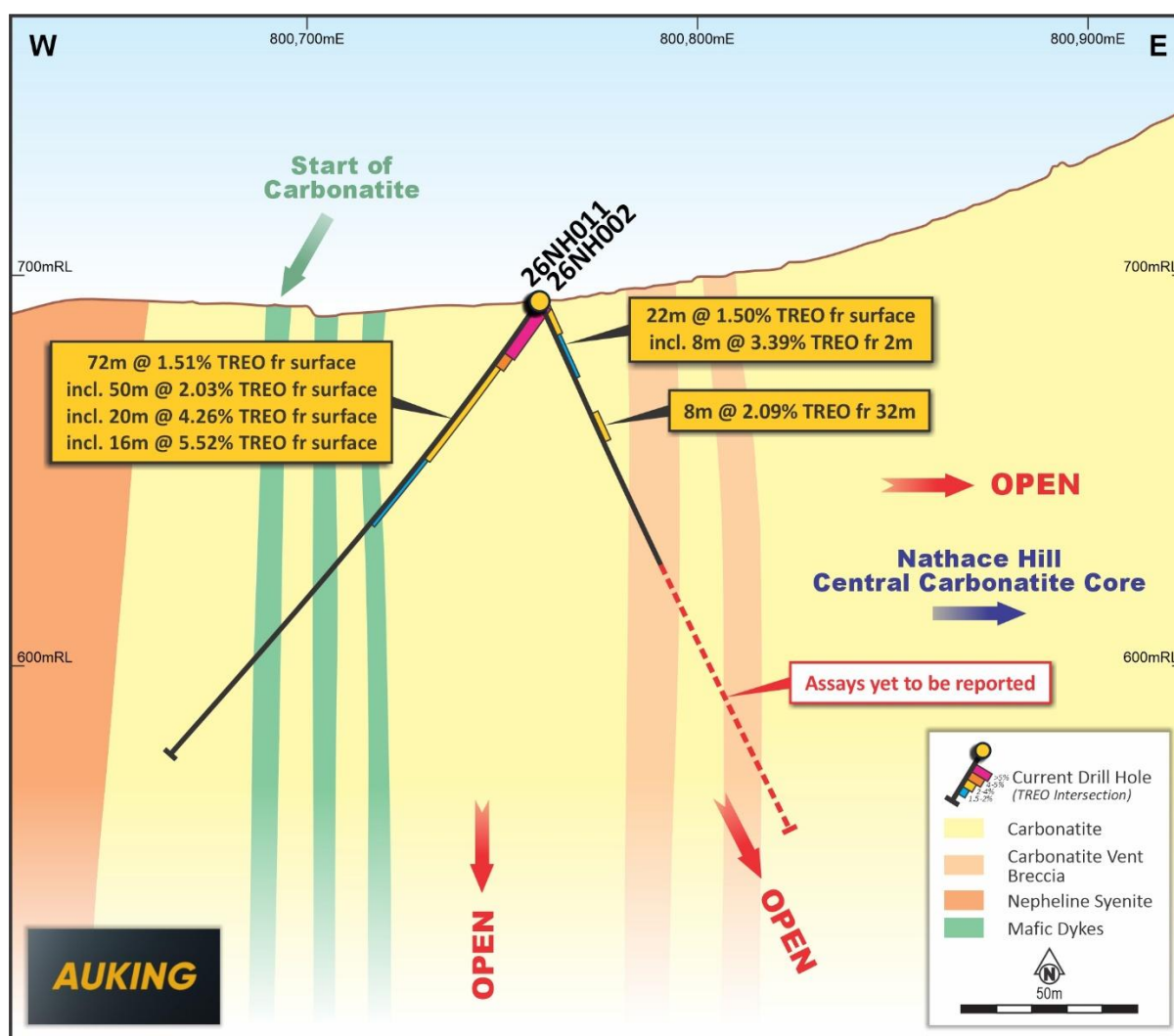
Figure 2 – Tundulu Drill holes 26NH002 and 26NH011 cross section
