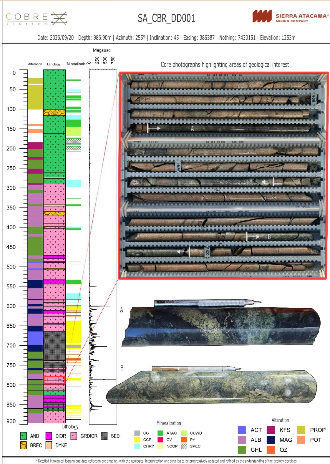
Figure 4. Graphical log with lithology and mineralisation, plus selected core photos. The supplied lithology and mineralisation graphic covers this.
