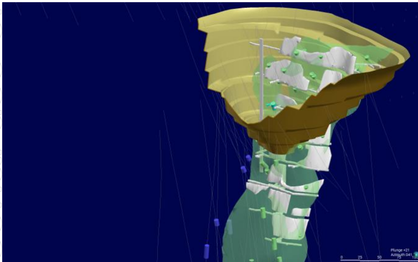
Figure 25: View from southwest of historic stopes (white), reserve pit (beige) and interpreted high grade (white) Source: ERM
