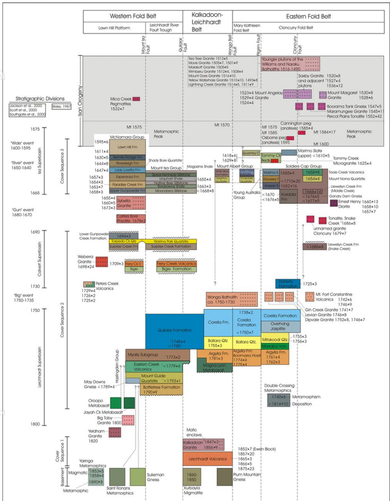
Figure 5: Stratigraphy of the Mount Isa Inlier
