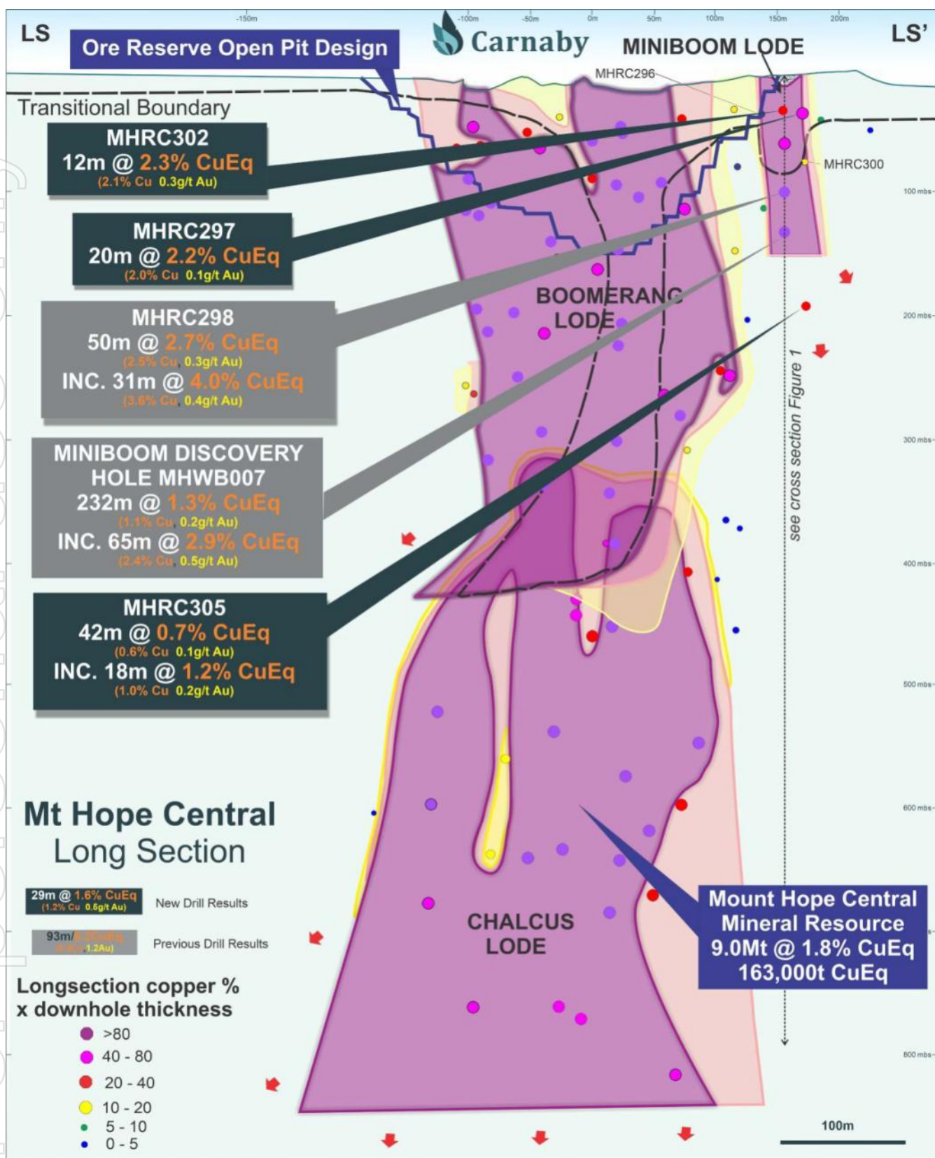
Figure 32: Mount Hope Central Long Section showing the new Miniboom Lodge Discovery Source: Carnaby (2026d)
