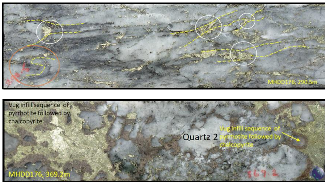
Figure 8: Quartz 1 (top) and Quartz 2 (bottom) style veining and sulphide mineralisation Source: Davis, 2023
