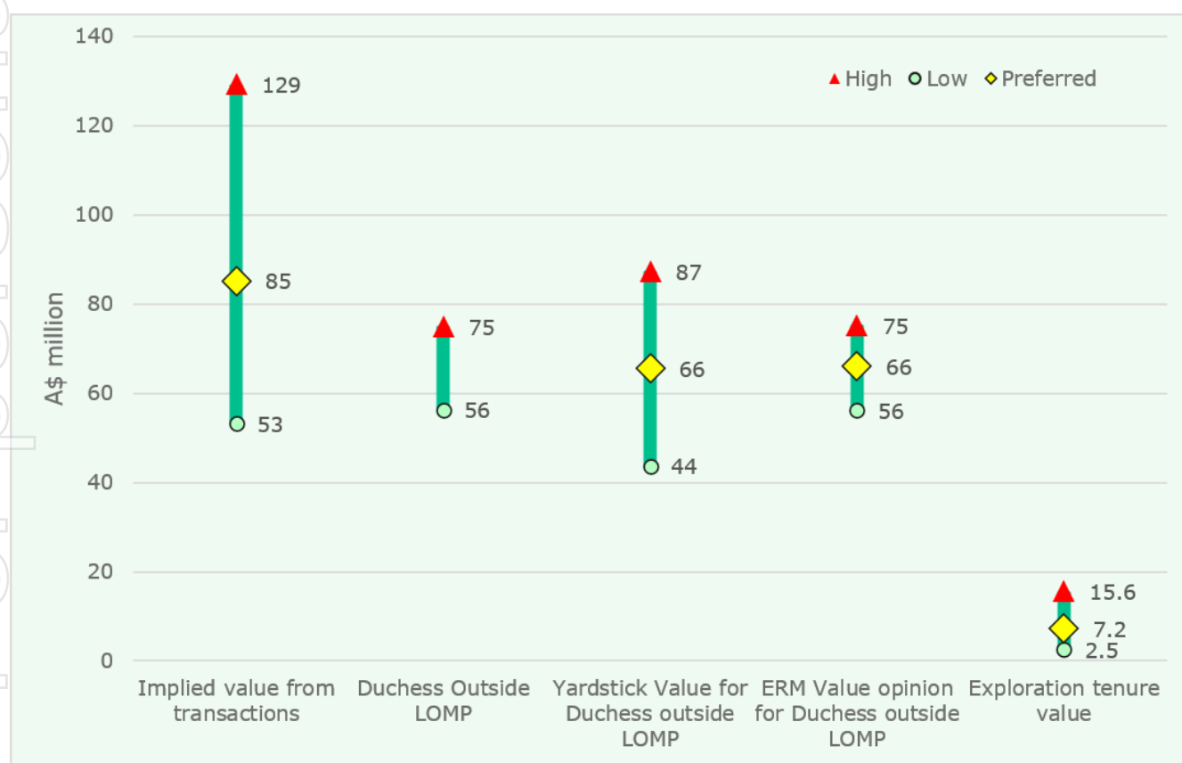
Figure 45: Valuation of Greater Duchess Copper Gold Project Mineral Resources less PFS Reserve component of the Resources
