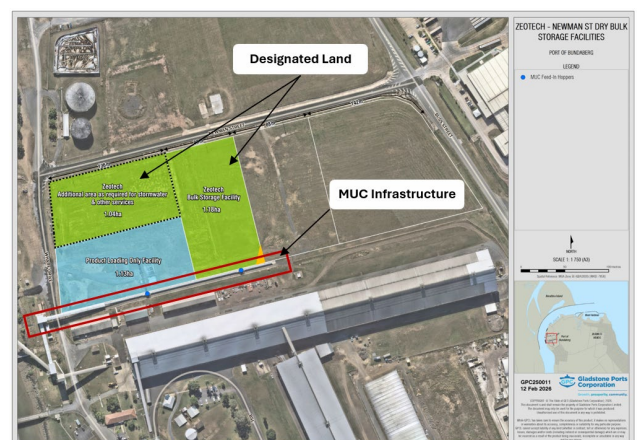
Figure 6: Proposed site (in green) for Zeotech's dry bulk Kaolin DSO receipt, storage and loading facility adjacent to the Multi-Use Conveyor (MUC) infrastructure at the Port of Bundaberg.
