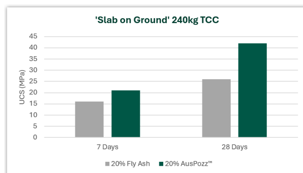
Figure 8: UCS of a reference mix design using Fly Ash (grey), compared with an AusPozz™ mix design (green) after 7 and 28 days
