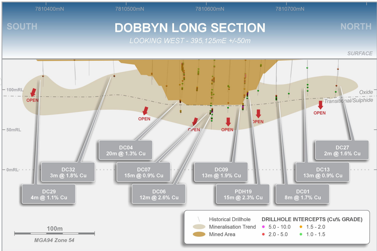
Figure 8. Dobbyn prospect long section (oblique view) showing drill hole intercepts and historic open pit.
