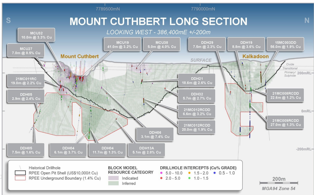
Figure 3. Mt Cuthbert-Kalkadoon deposits long section showing Mineral Resource category, drill hole intercepts and historic pits.
