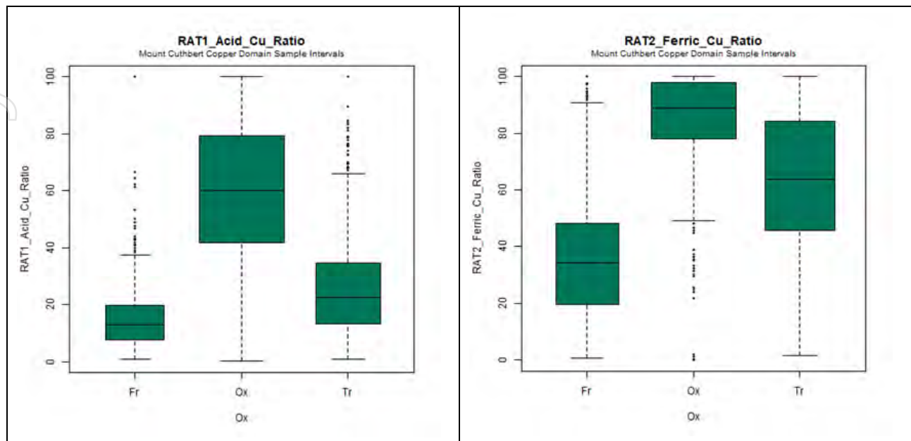
Figure 8-5. Acid-soluble (LHS) and ferric-soluble (RHS) copper ratios by ore type.
