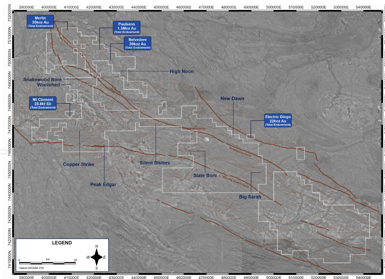
Figure 4: Map of the greater Paulsens Gold Operation showing regional gold prospects and known deposits with total endowment indicated (historical production plus current Resource).
