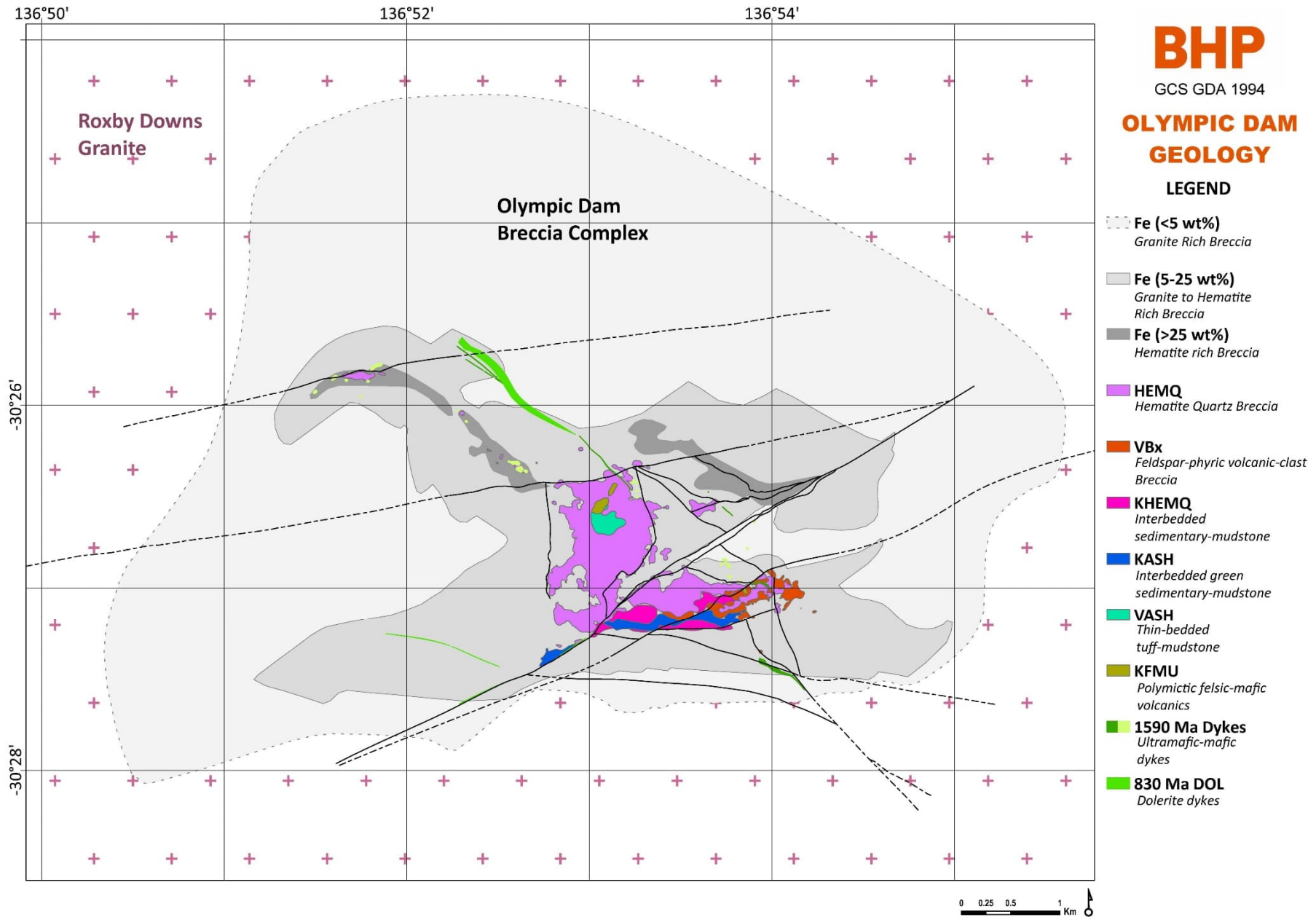
Figure 3. Simplified geological plan of the Olympic Dam deposit, approximately 350 m below surface.
