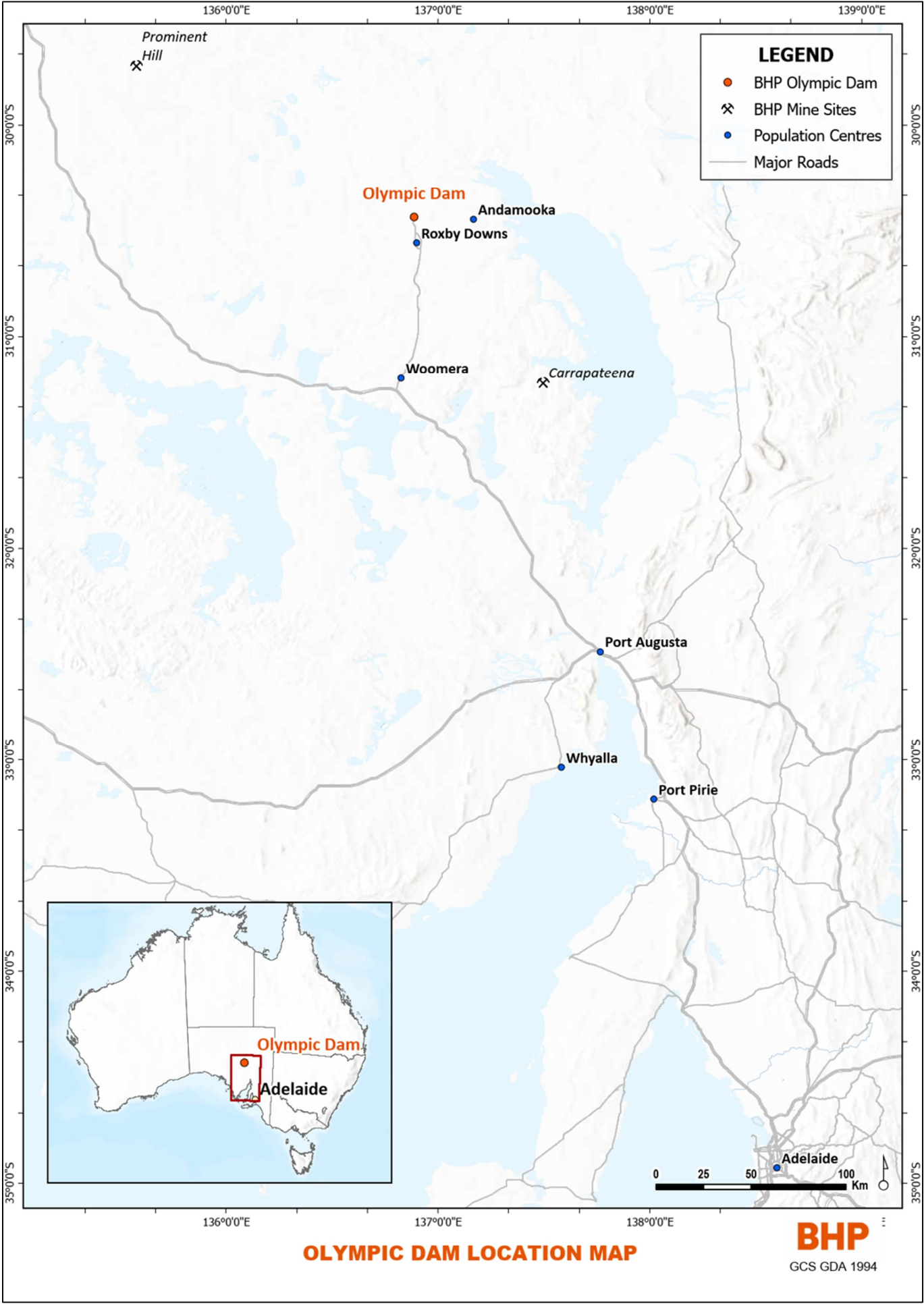
Figure 1. Location of the Olympic Dam mine.
