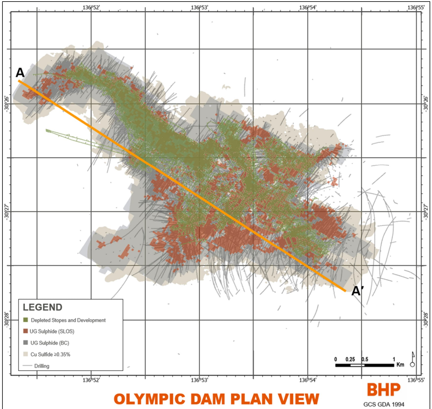
Figure 4. Plan view of the Olympic Dam deposit, showing the spatial relationship between a 0.35% Cu envelope, the outlines of mineral resource block cave and sublevel stoping. Mined stope, development and drilling provided for context.
