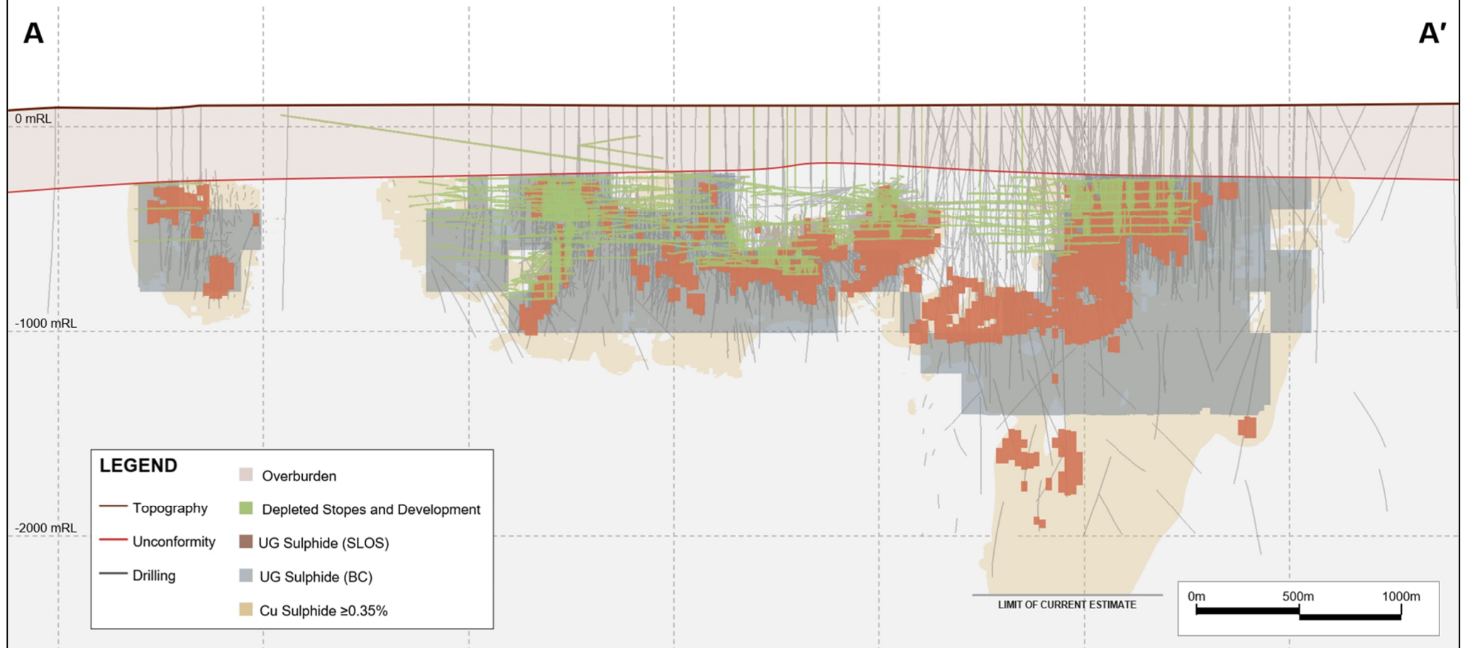
Figure 5. Long section through the Olympic Dam deposit along A – A' (Figure 4) looking NE. The ~500 m thick projection shows the spatial relationship between a 0.35% Cu envelope, the outlines of mineral resource block cave and sublevel stoping. Mined stope, development and drilling provided for context
