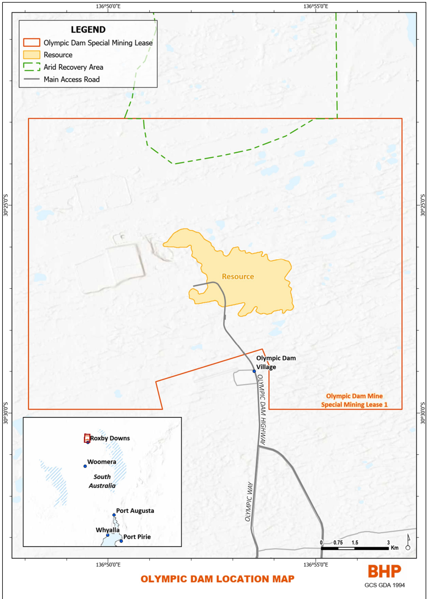
Figure 2. Approximate Olympic Dam resource outline within Special Mining Lease 1 (SML)
